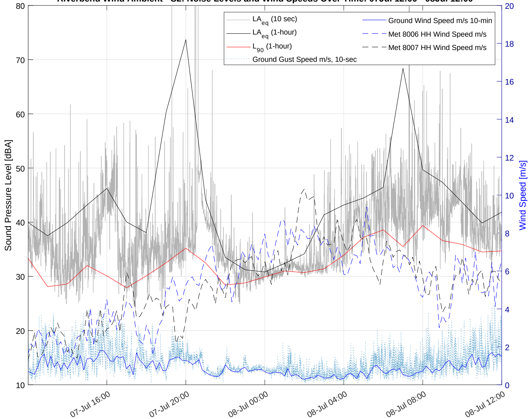
Riverbend Wind Ambient - S2: Noise Levels and Wind Speeds Over Time: 07Jul 12:00 - 08Jul 12:00
