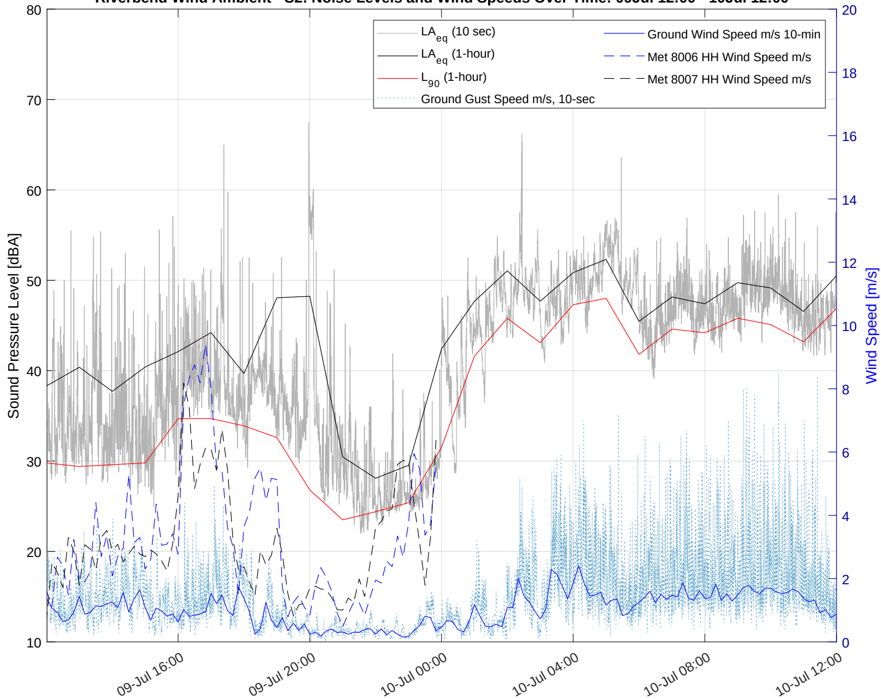
Riverbend Wind Ambient - S2: Noise Levels and Wind Speeds Over Time: 09Jul 12:00 - 10Jul 12:00
