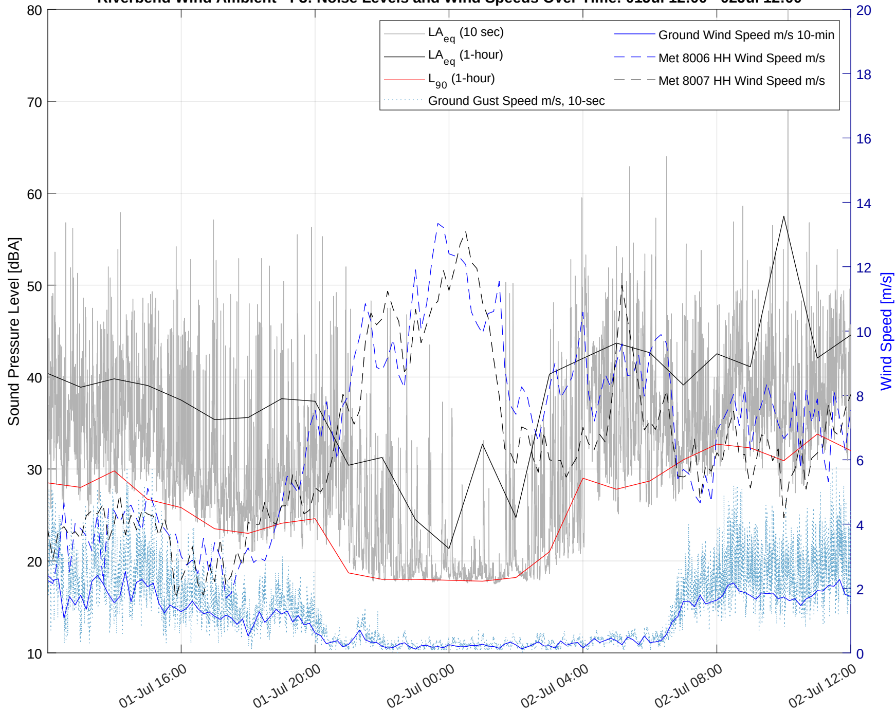
Riverbend Wind Ambient - F3: Noise Levels and Wind Speeds Over Time: 01Jul 12:00 - 02Jul 12:00
