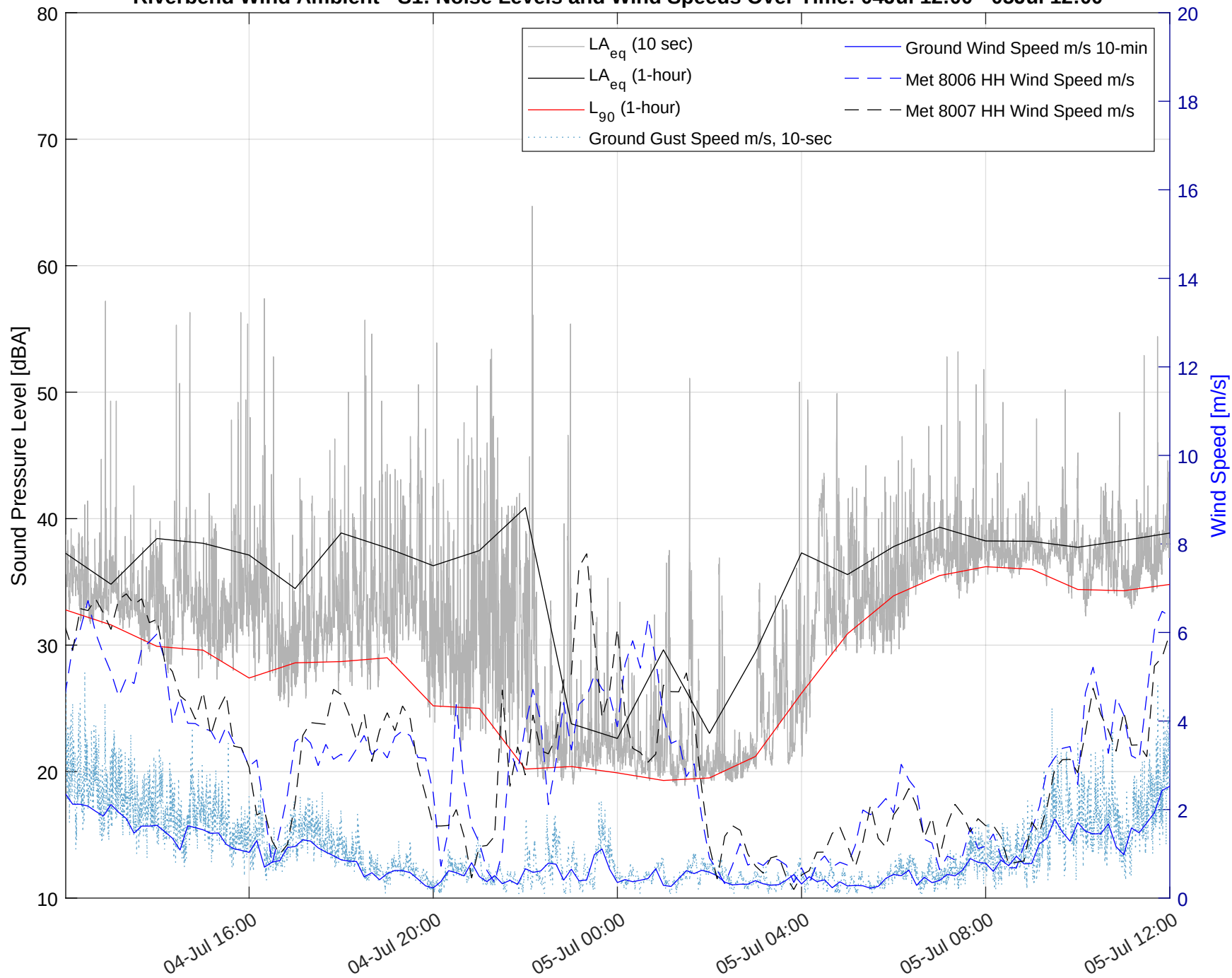
Riverbend Wind Ambient - S1: Noise Levels and Wind Speeds Over Time: 04Jul 12:00 - 05Jul 12:00
