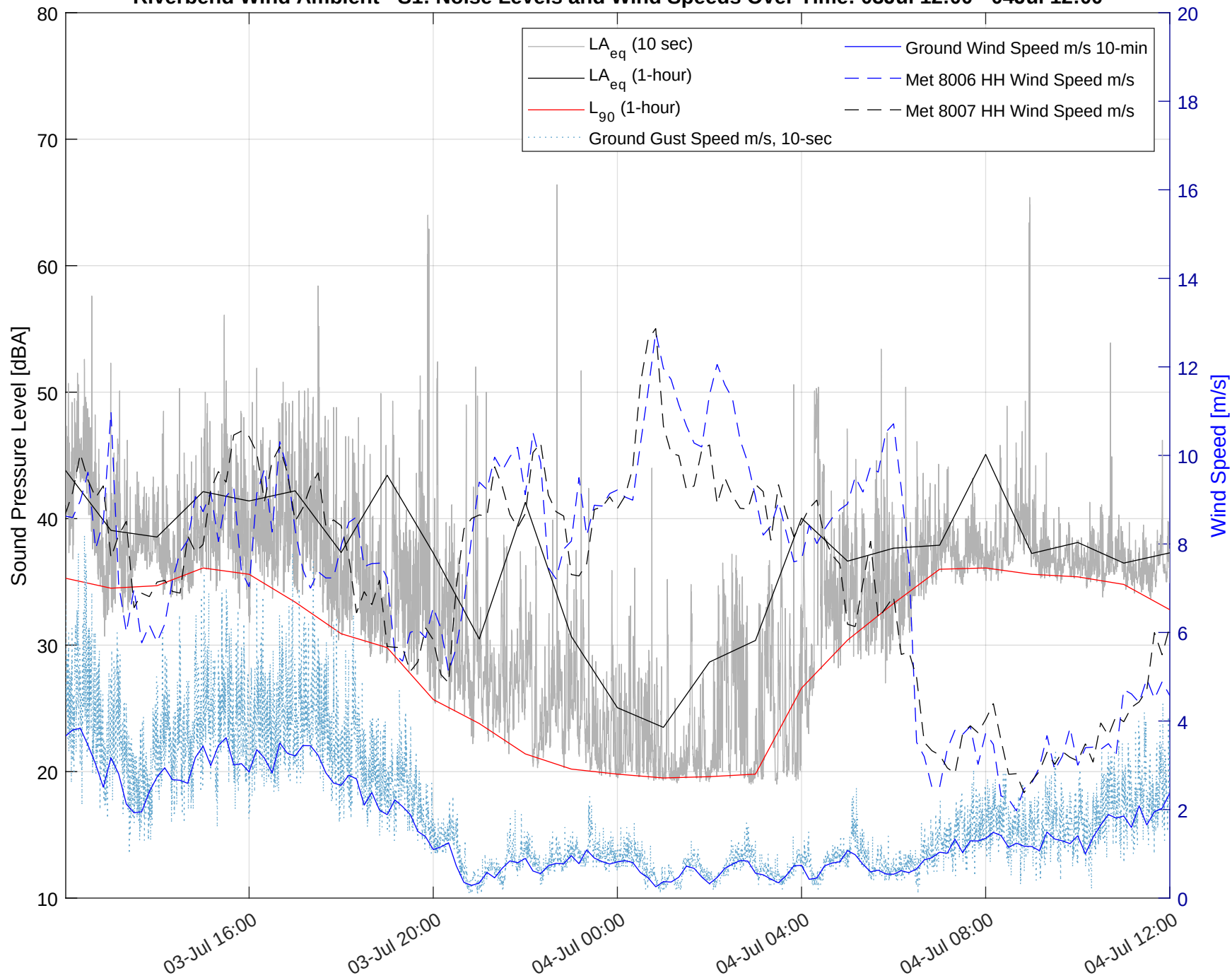
Riverbend Wind Ambient - S1: Noise Levels and Wind Speeds Over Time: 03Jul 12:00 - 04Jul 12:00
