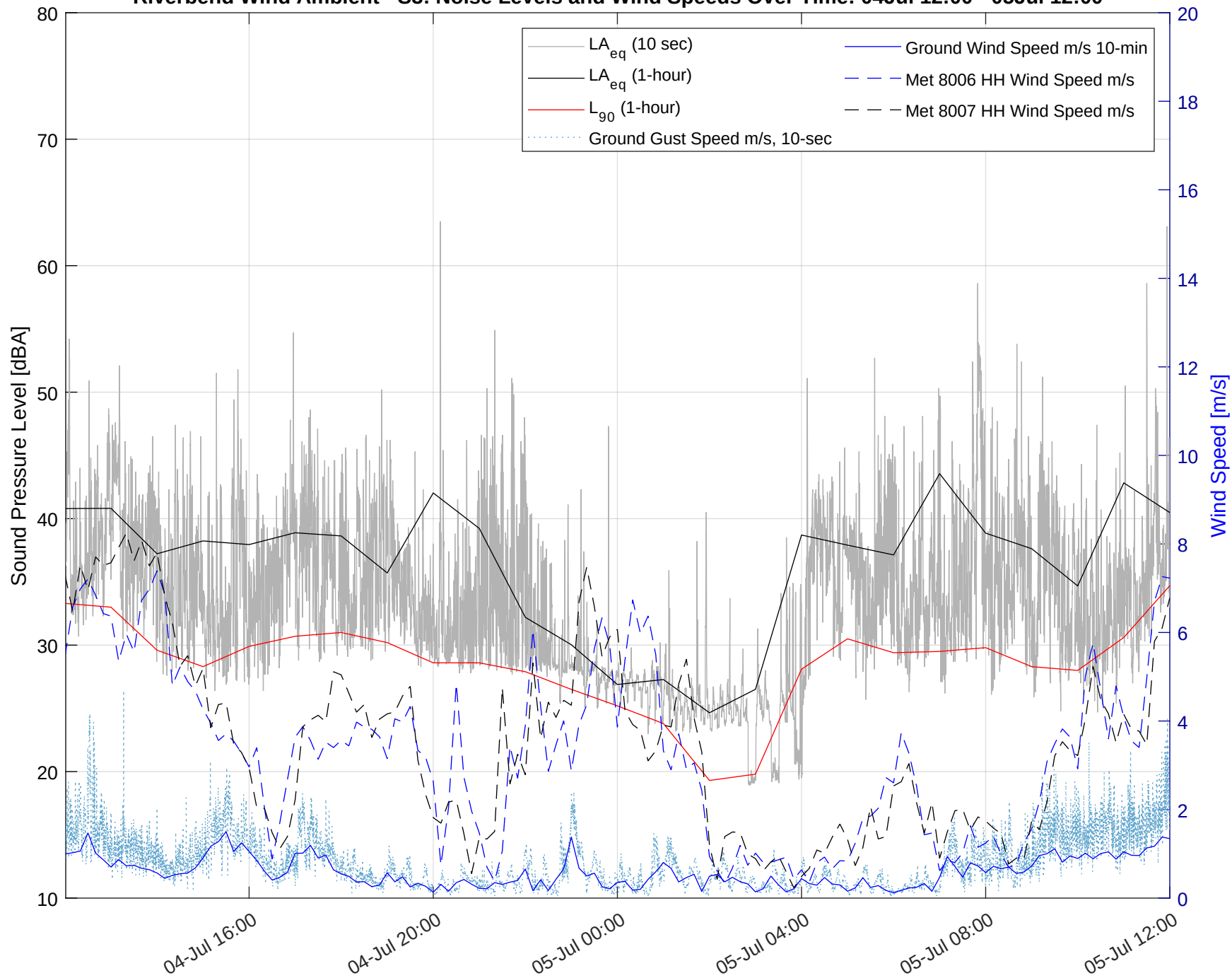
Riverbend Wind Ambient - S3: Noise Levels and Wind Speeds Over Time: 04Jul 12:00 - 05Jul 12:00
