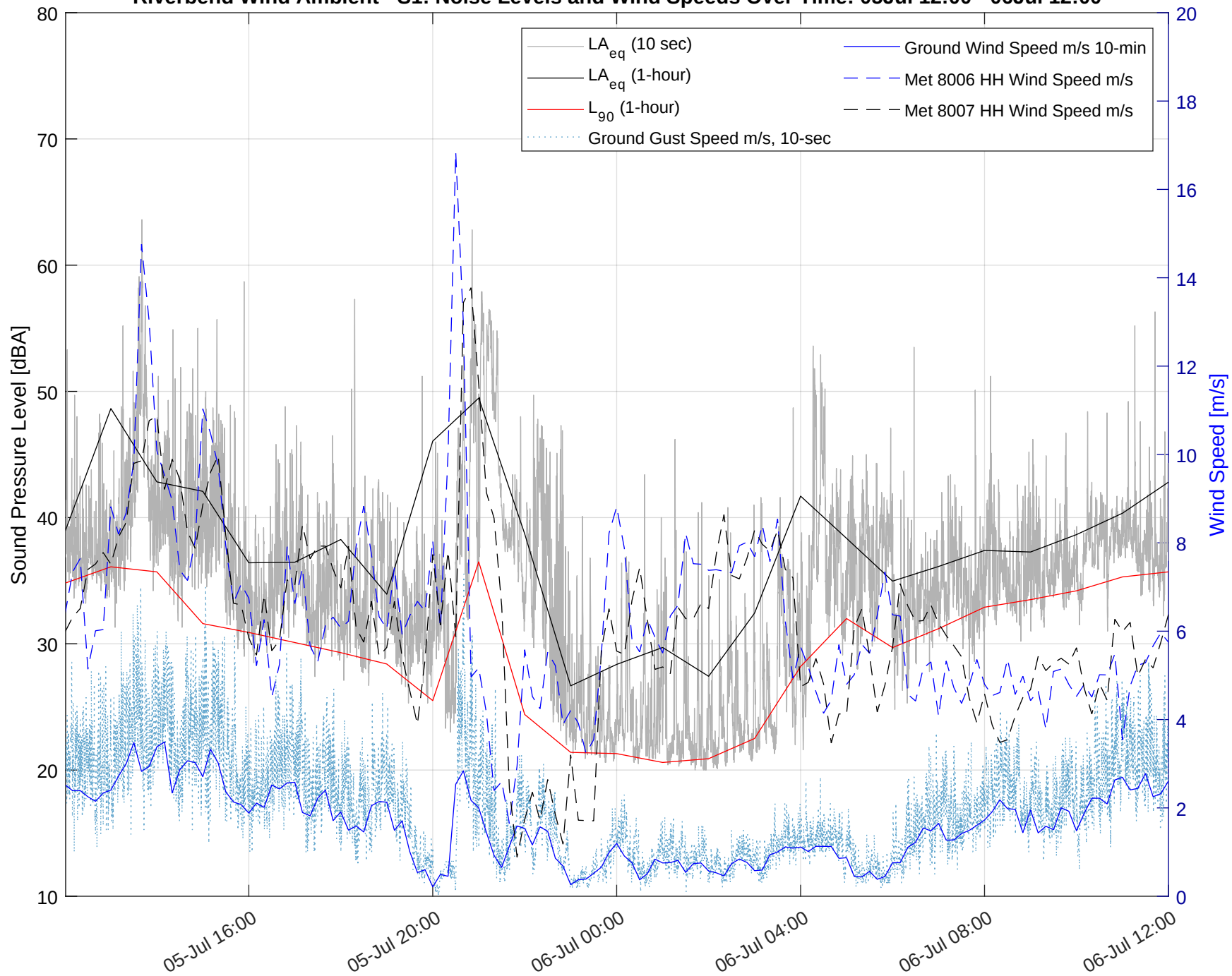
Riverbend Wind Ambient - S1: Noise Levels and Wind Speeds Over Time: 05Jul 12:00 - 06Jul 12:00
