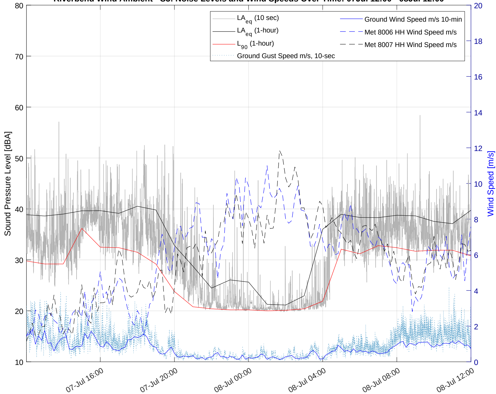
Riverbend Wind Ambient - S3: Noise Levels and Wind Speeds Over Time: 07Jul 12:00 - 08Jul 12:00
