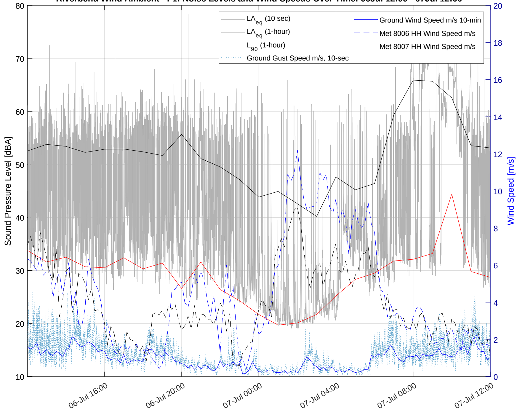
Riverbend Wind Ambient - F1: Noise Levels and Wind Speeds Over Time: 06Jul 12:00 - 07Jul 12:00
