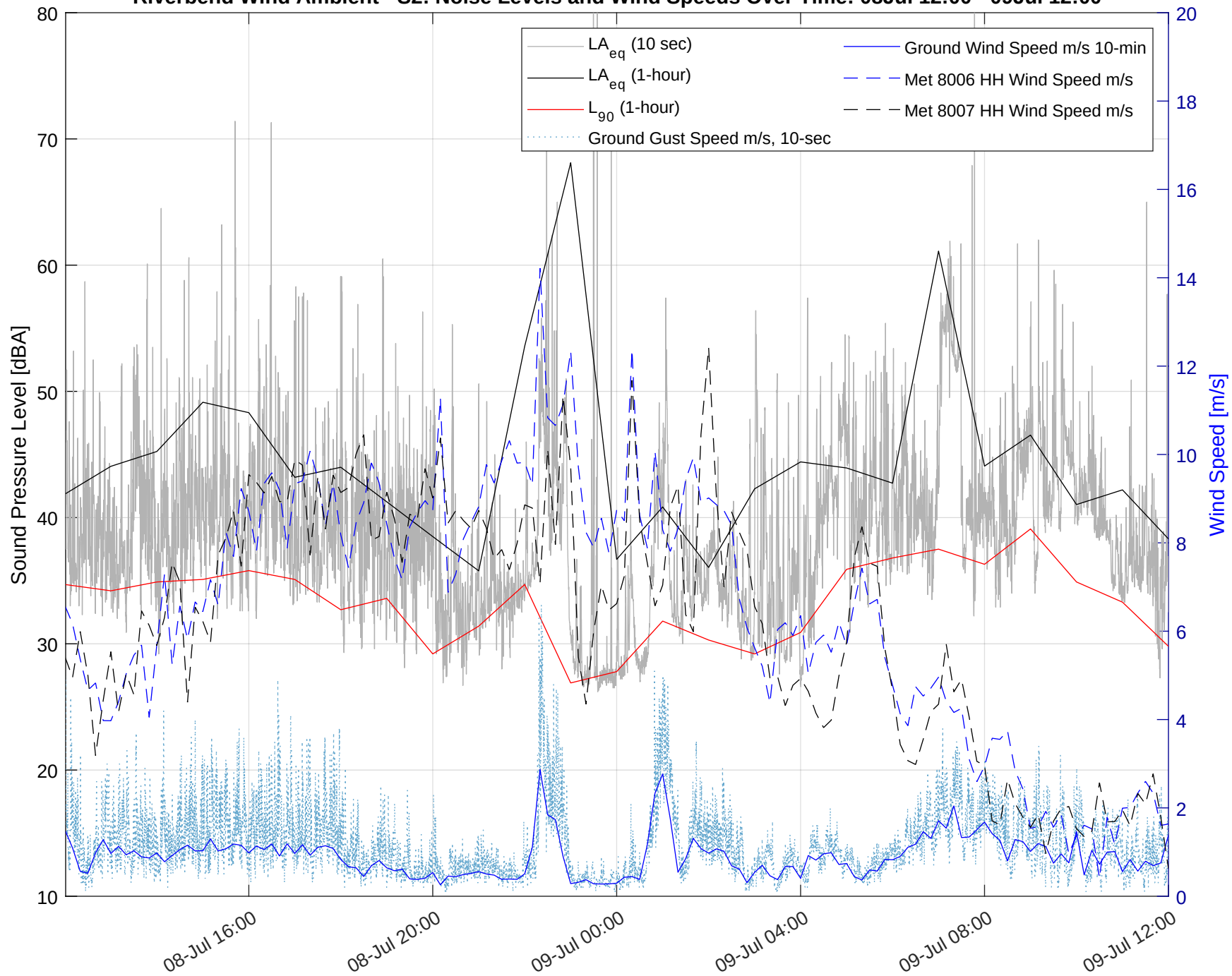
Riverbend Wind Ambient - S2: Noise Levels and Wind Speeds Over Time: 08Jul 12:00 - 09Jul 12:00
