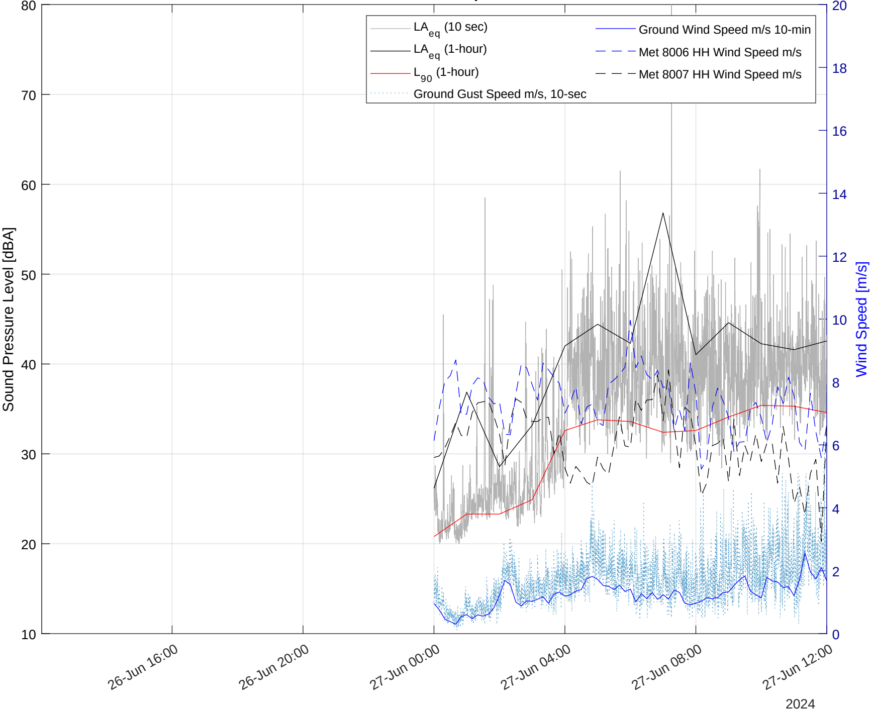
Riverbend Wind Ambient - F3: Noise Levels and Wind Speeds Over Time: 26Jun 12:00 - 27Jun 12:00
