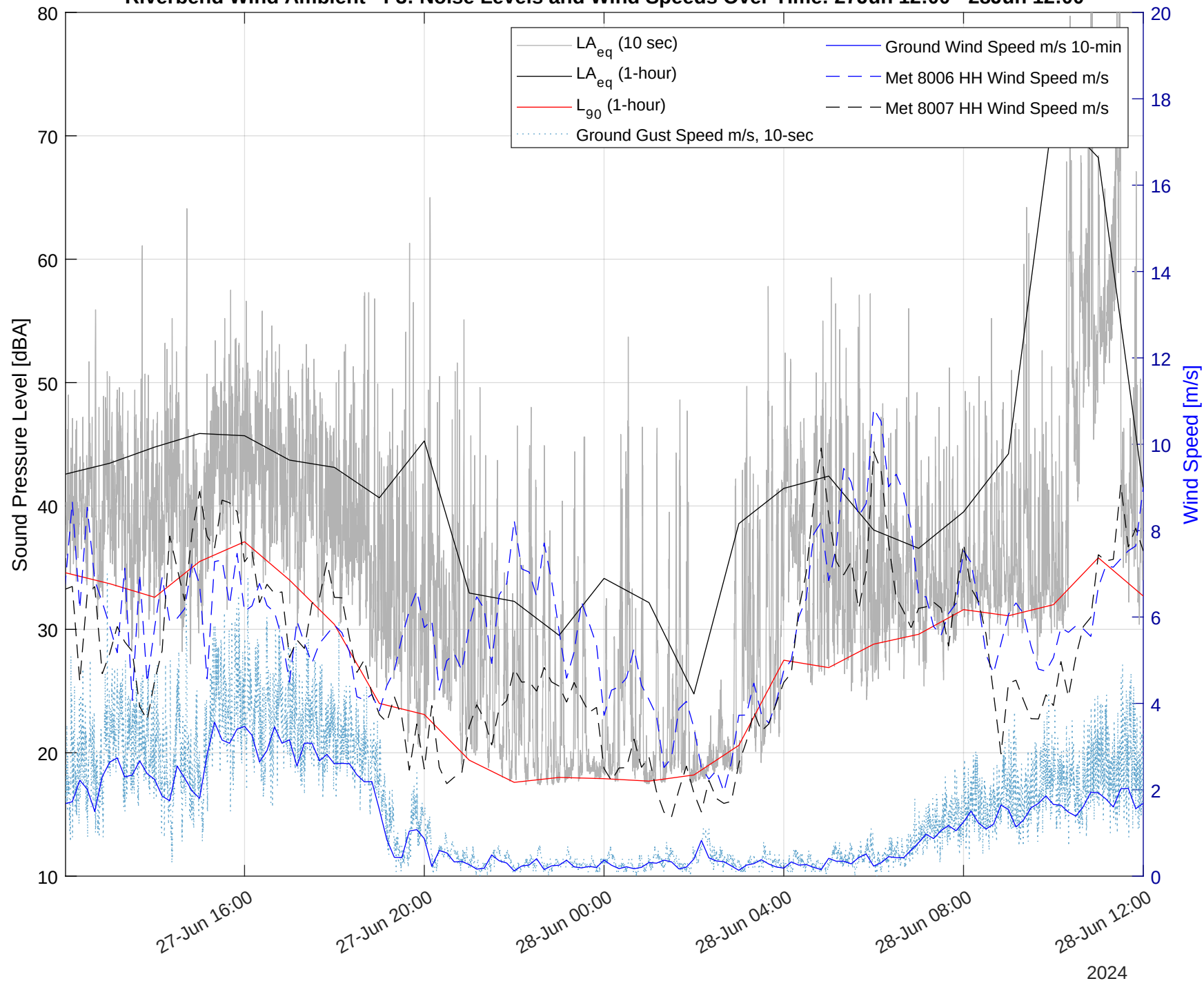
Riverbend Wind Ambient - F3: Noise Levels and Wind Speeds Over Time: 27Jun 12:00 - 28Jun 12:00
