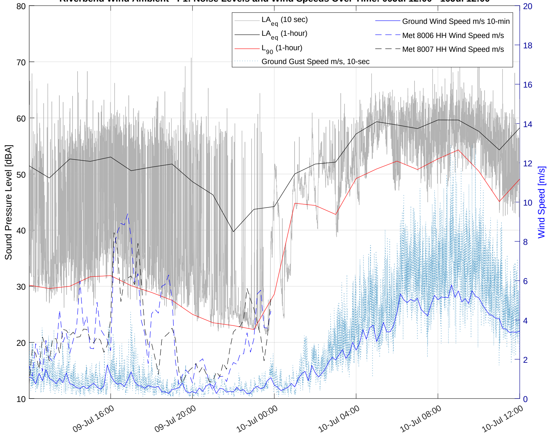
Riverbend Wind Ambient - F1: Noise Levels and Wind Speeds Over Time: 09Jul 12:00 - 10Jul 12:00
