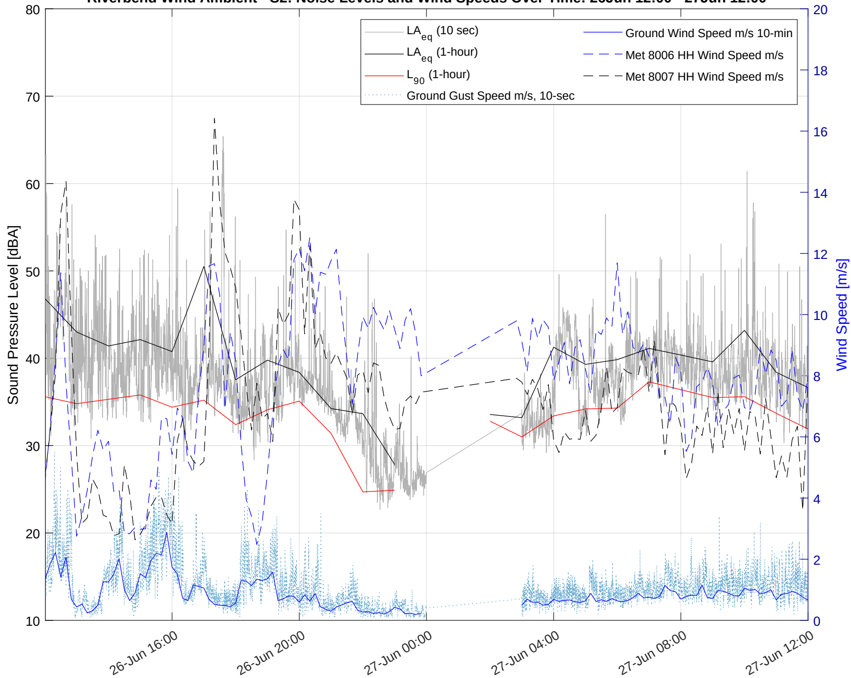
Riverbend Wind Ambient - S2: Noise Levels and Wind Speeds Over Time: 26Jun 12:00 - 27Jun 12:00
