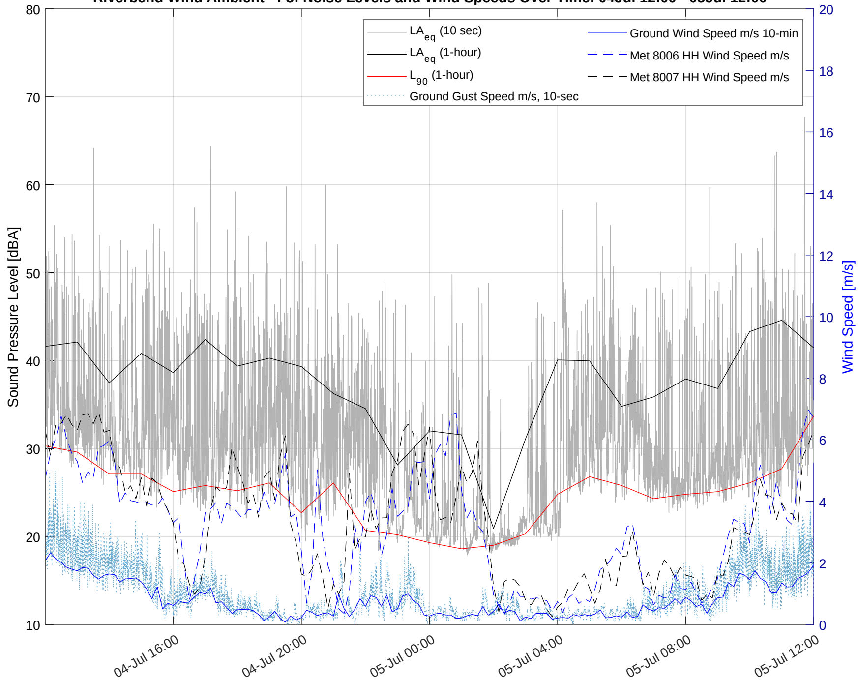
Riverbend Wind Ambient - F3: Noise Levels and Wind Speeds Over Time: 04Jul 12:00 - 05Jul 12:00
