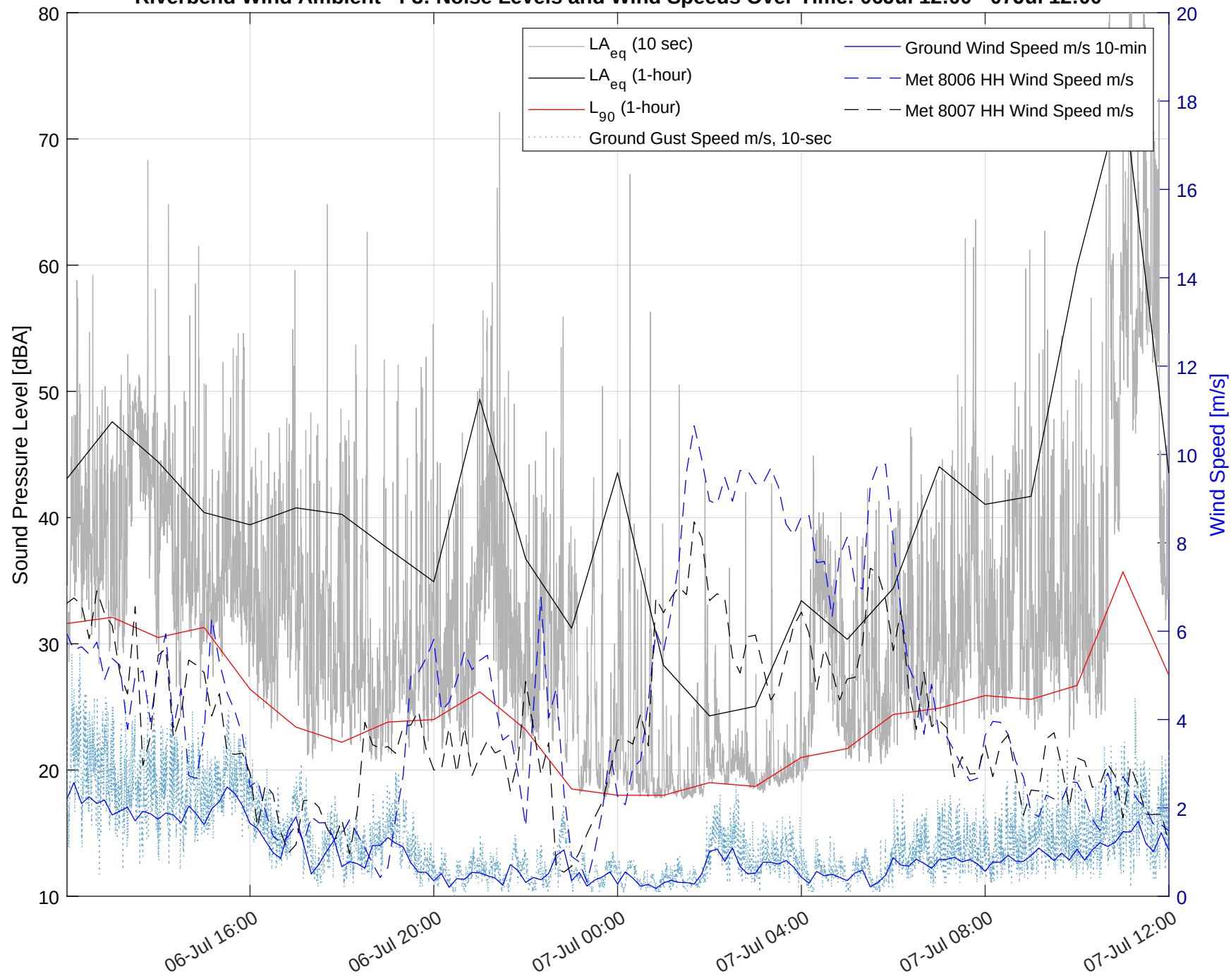
Riverbend Wind Ambient - F3: Noise Levels and Wind Speeds Over Time: 06Jul 12:00 - 07Jul 12:00
