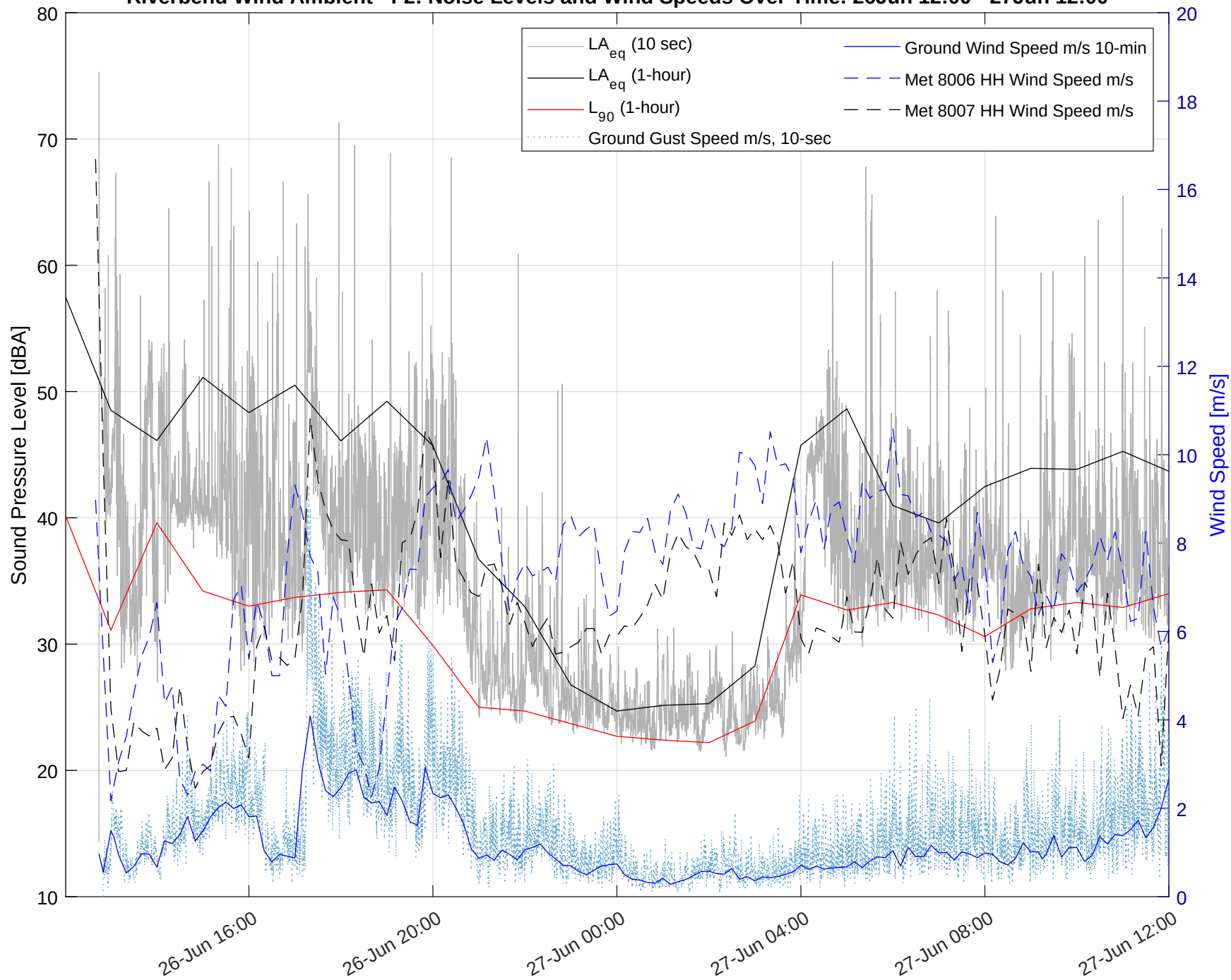
Riverbend Wind Ambient - F2: Noise Levels and Wind Speeds Over Time: 26Jun 12:00 - 27Jun 12:00
