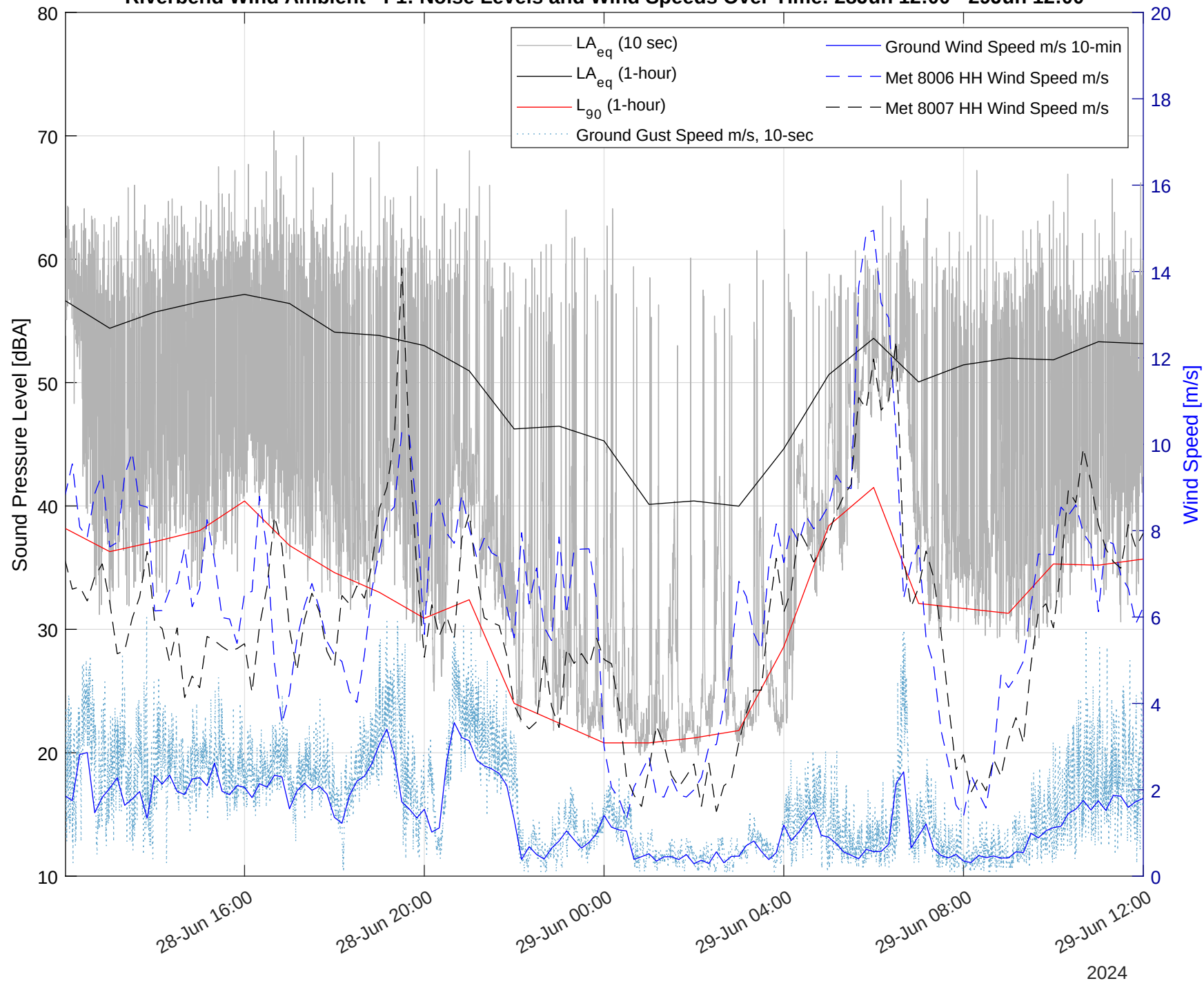
Riverbend Wind Ambient - F1: Noise Levels and Wind Speeds Over Time: 28Jun 12:00 - 29Jun 12:00
