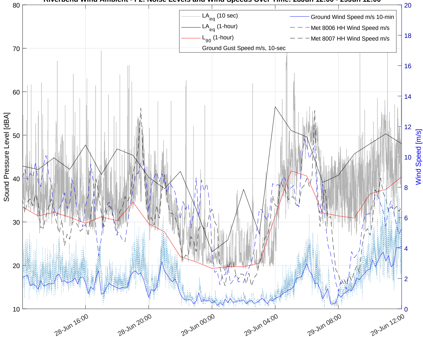
Riverbend Wind Ambient - F2: Noise Levels and Wind Speeds Over Time: 28Jun 12:00 - 29Jun 12:00
