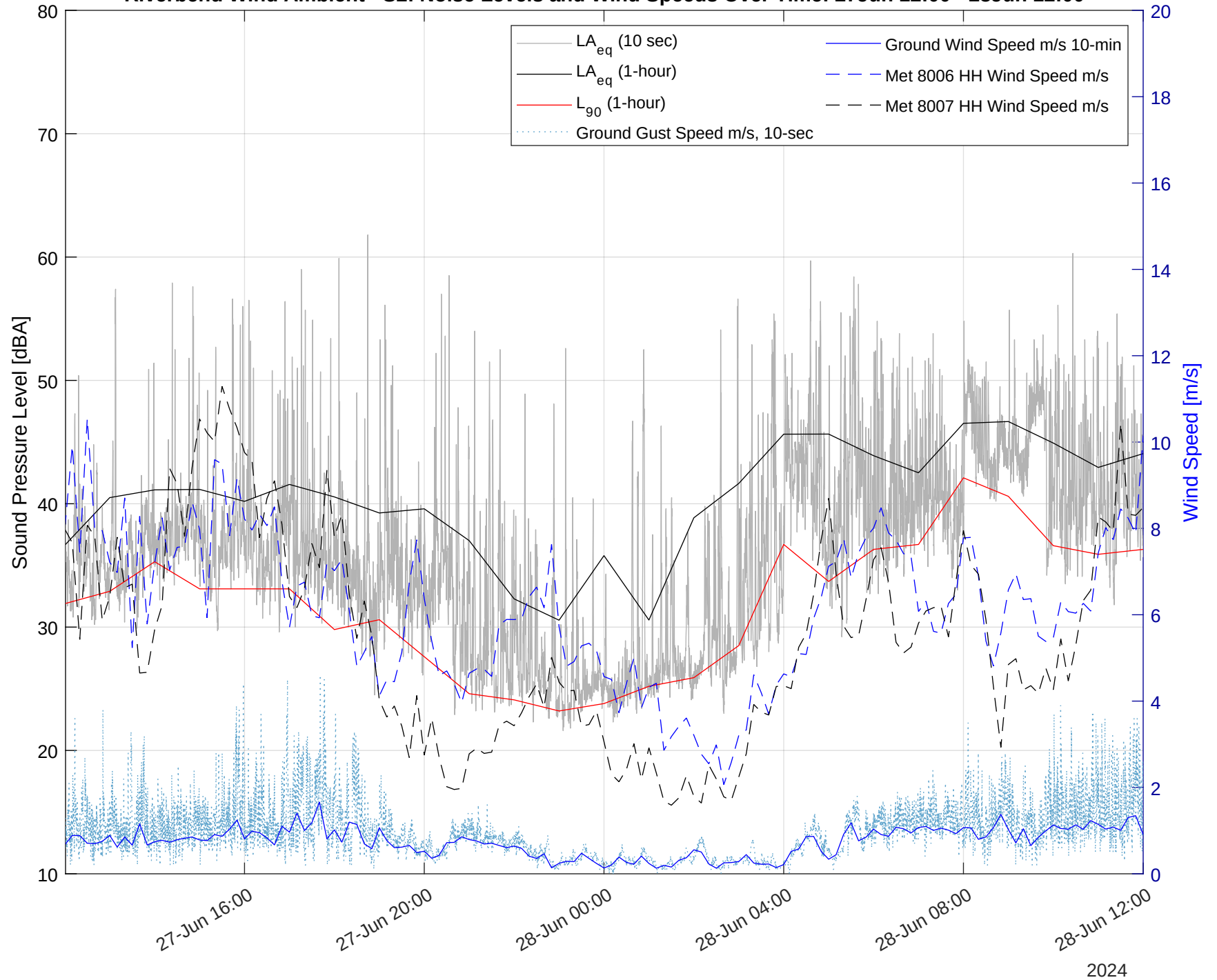
Riverbend Wind Ambient - S2: Noise Levels and Wind Speeds Over Time: 27Jun 12:00 - 28Jun 12:00
