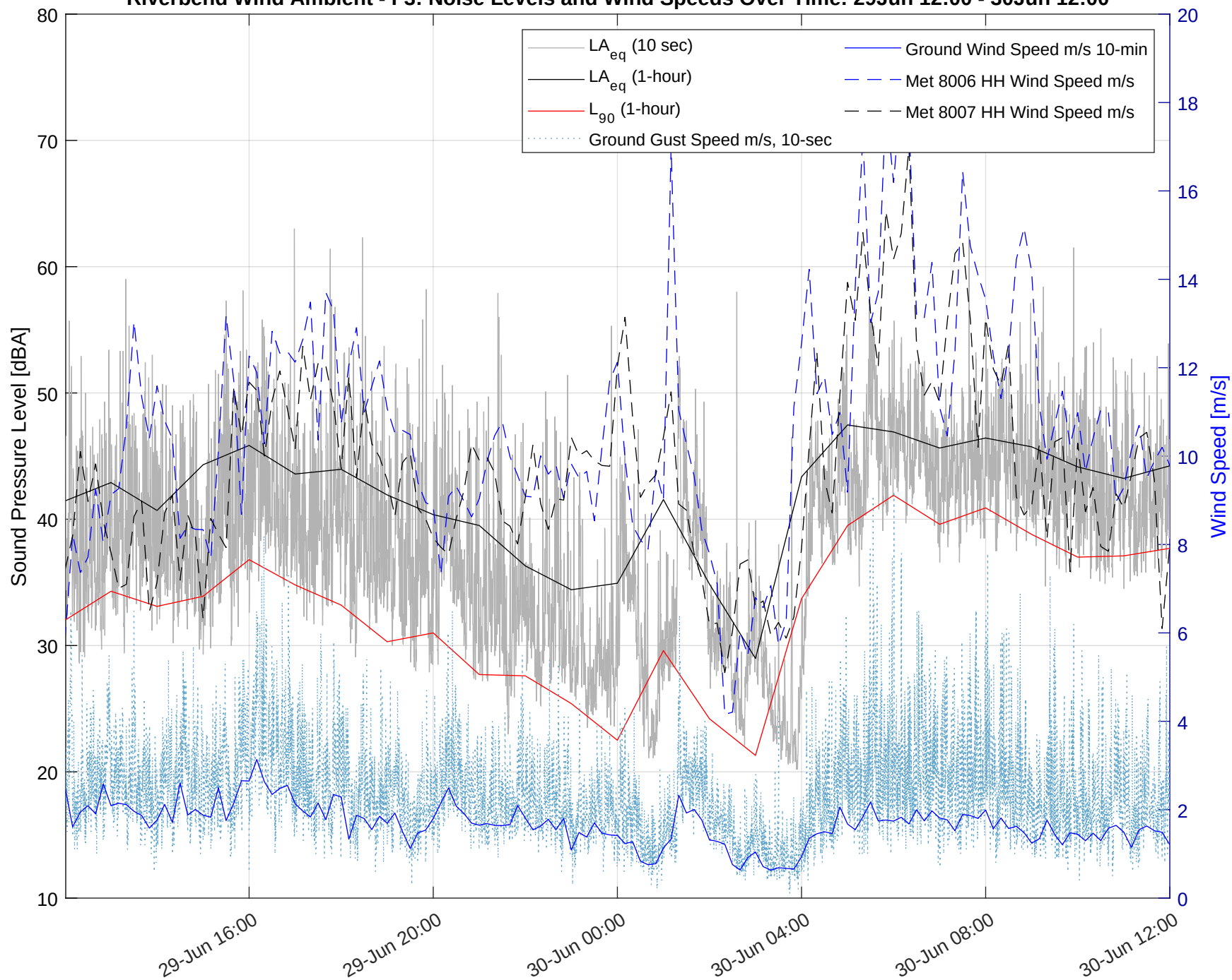
Riverbend Wind Ambient - F3: Noise Levels and Wind Speeds Over Time: 29Jun 12:00 - 30Jun 12:00
