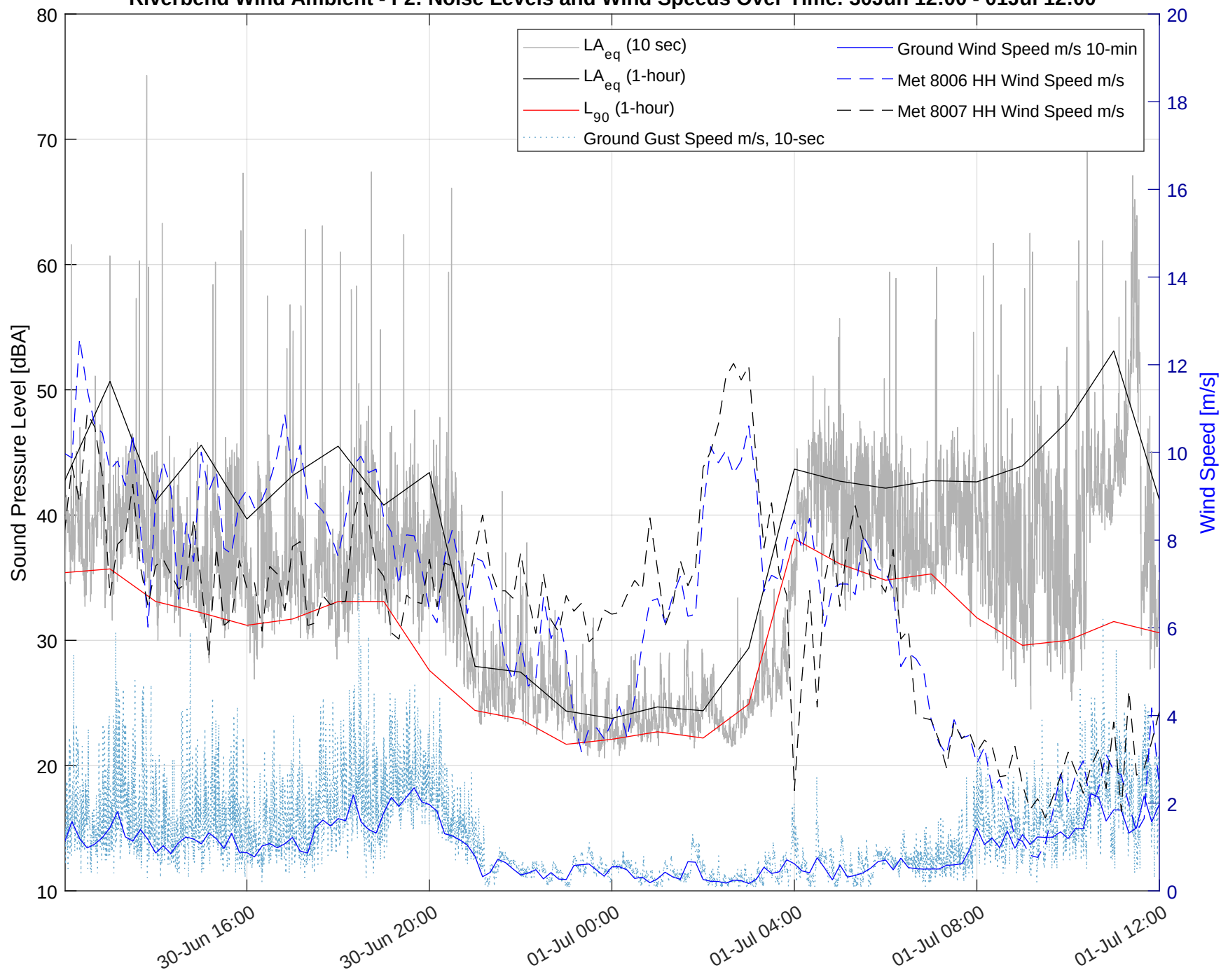
Riverbend Wind Ambient - F2: Noise Levels and Wind Speeds Over Time: 30Jun 12:00 - 01Jul 12:00
