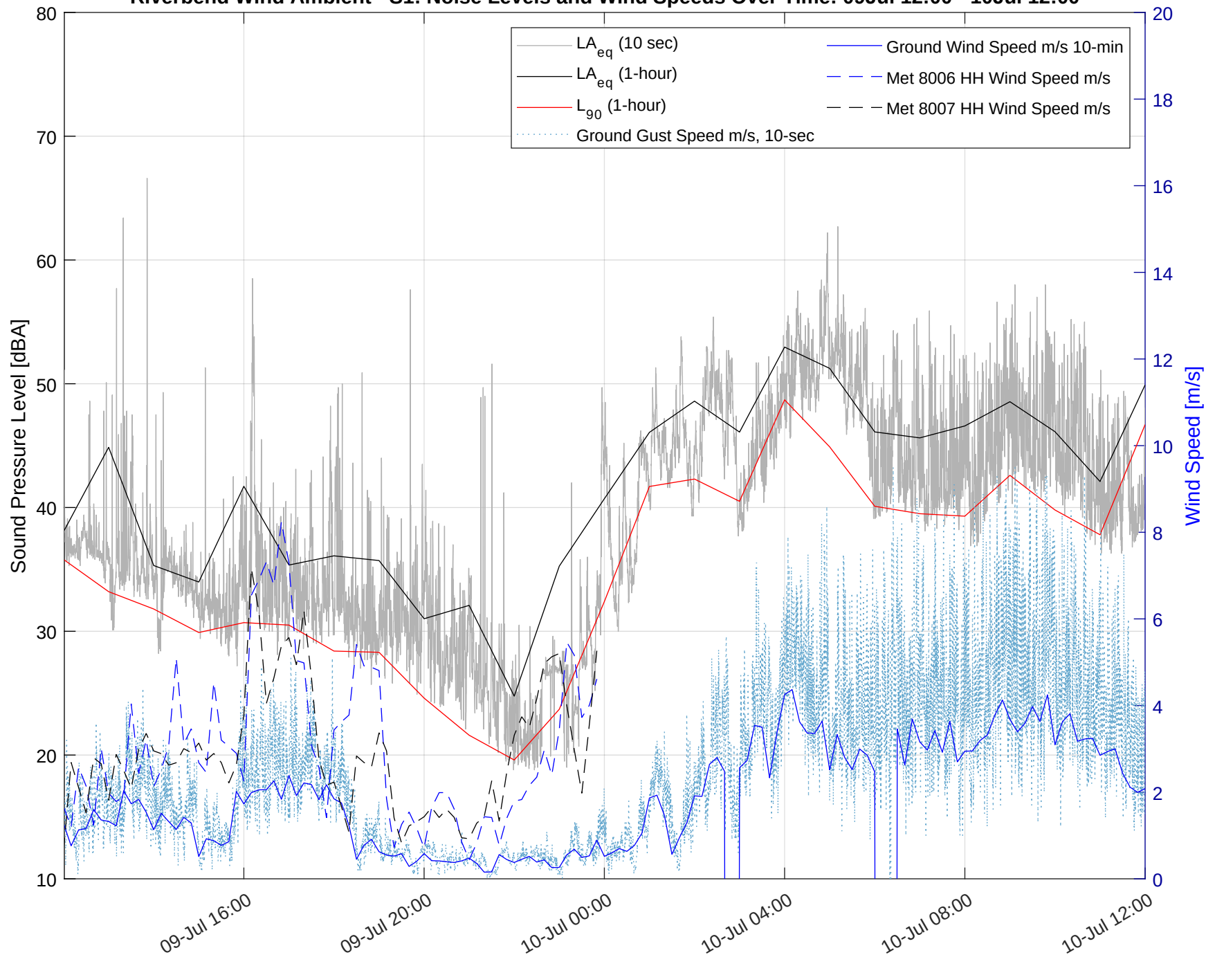
Riverbend Wind Ambient - S1: Noise Levels and Wind Speeds Over Time: 09Jul 12:00 - 10Jul 12:00
