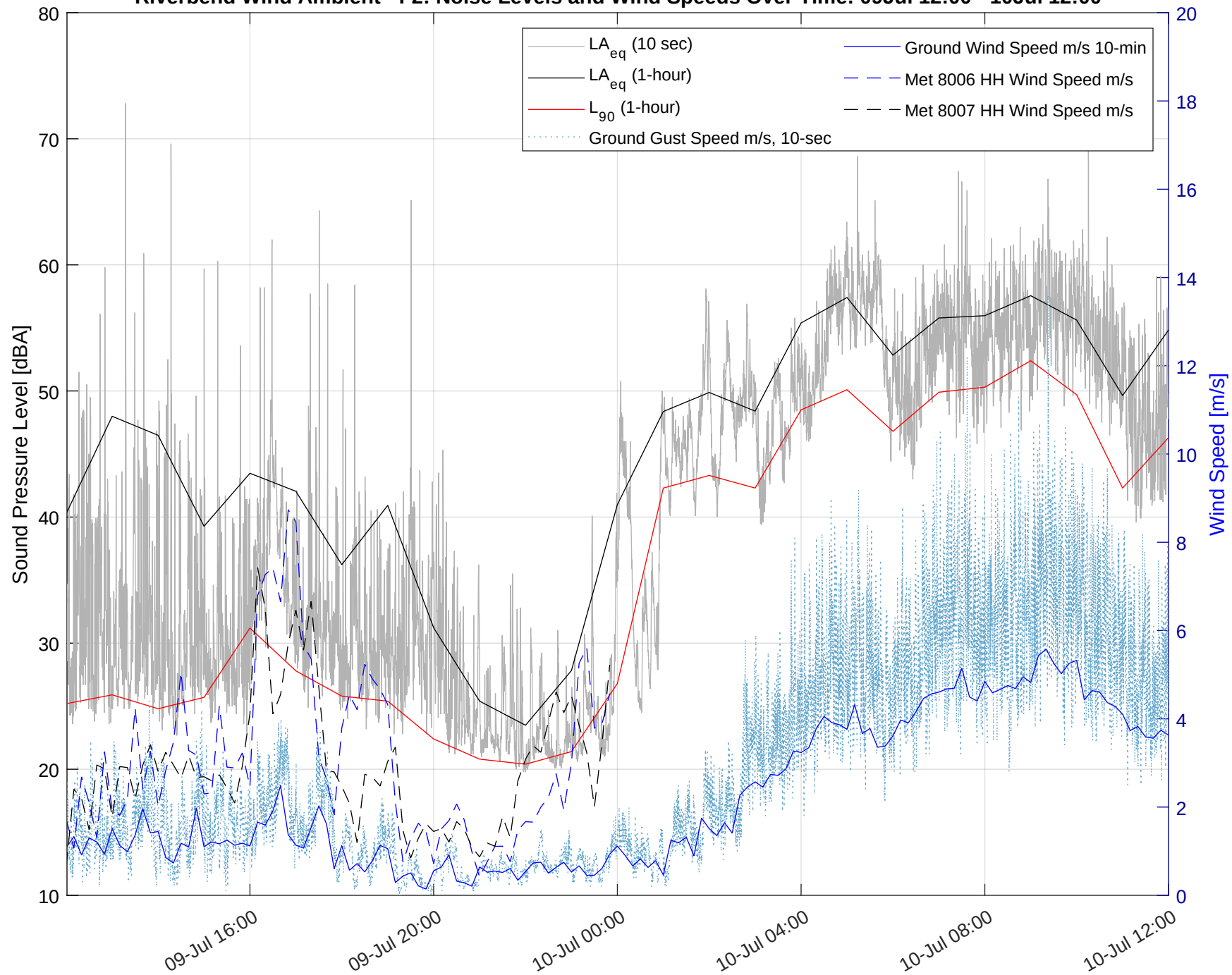
Riverbend Wind Ambient - F2: Noise Levels and Wind Speeds Over Time: 09Jul 12:00 - 10Jul 12:00
