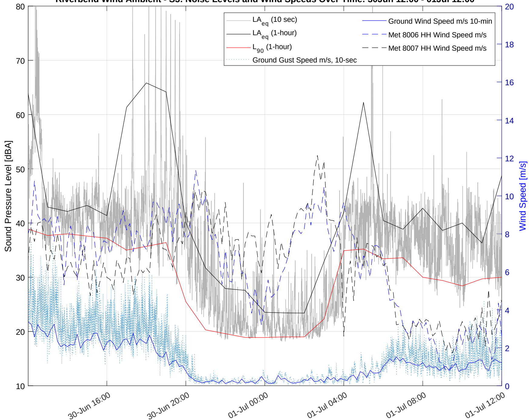
Riverbend Wind Ambient - S3: Noise Levels and Wind Speeds Over Time: 30Jun 12:00 - 01Jul 12:00
