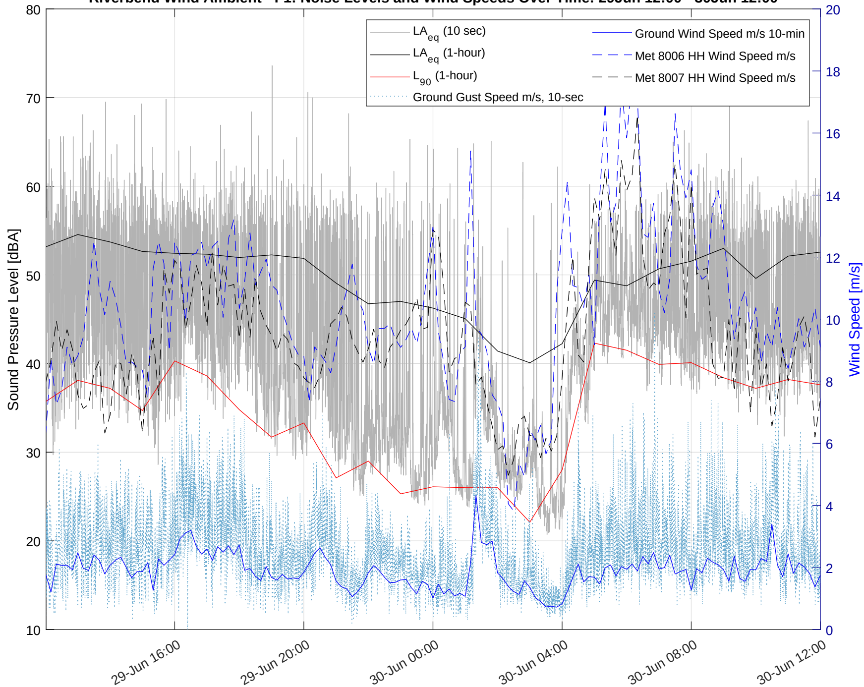
Riverbend Wind Ambient - F1: Noise Levels and Wind Speeds Over Time: 29Jun 12:00 - 30Jun 12:00
