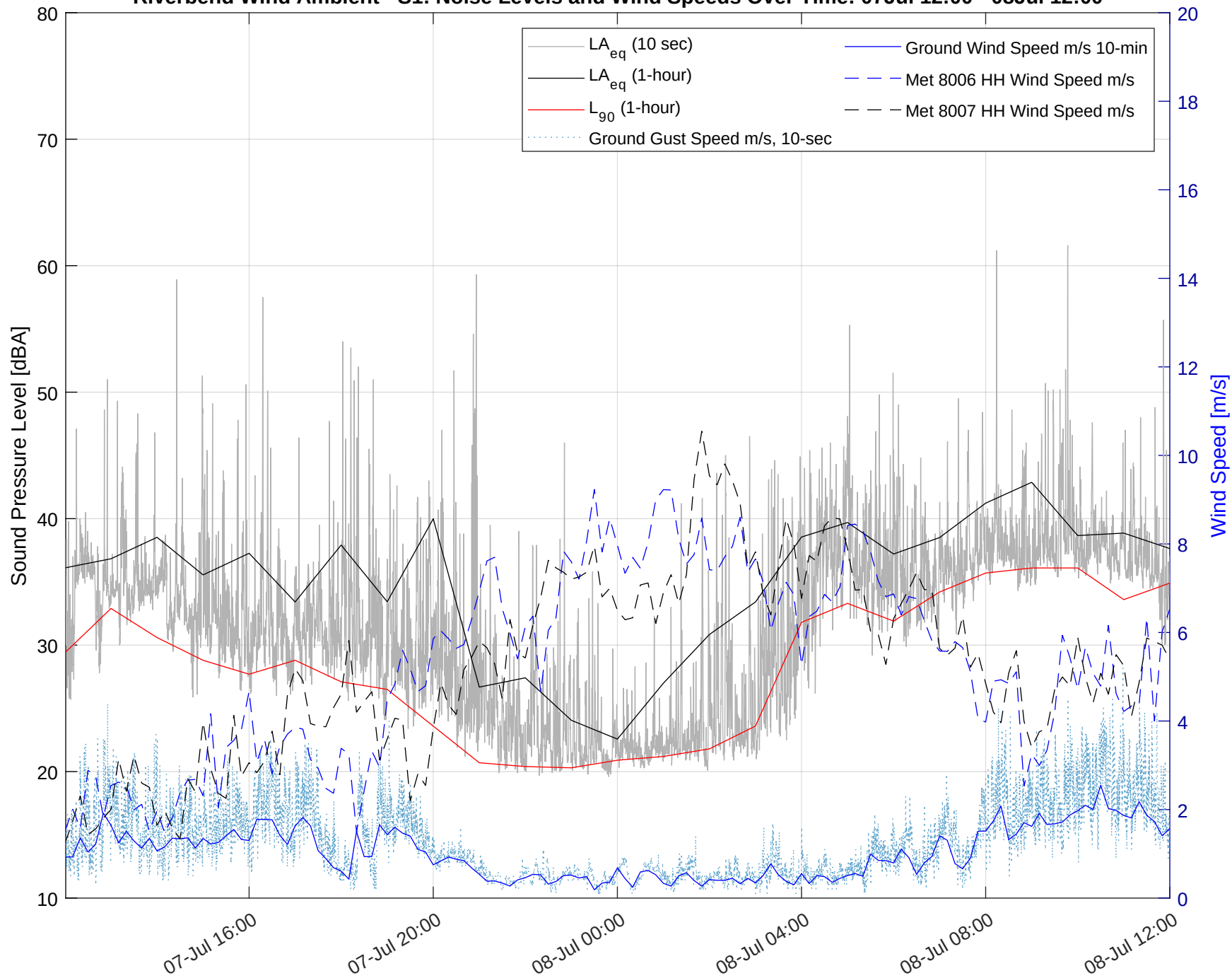
Riverbend Wind Ambient - S1: Noise Levels and Wind Speeds Over Time: 07Jul 12:00 - 08Jul 12:00
