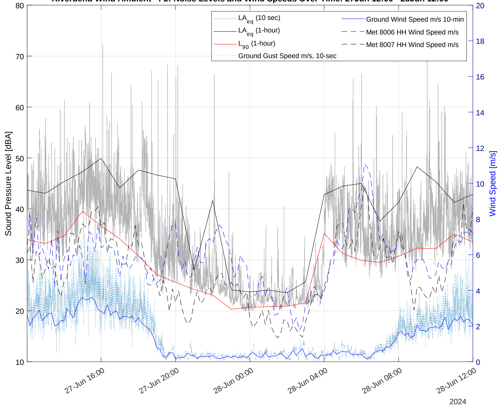
Riverbend Wind Ambient - F2: Noise Levels and Wind Speeds Over Time: 27Jun 12:00 - 28Jun 12:00
