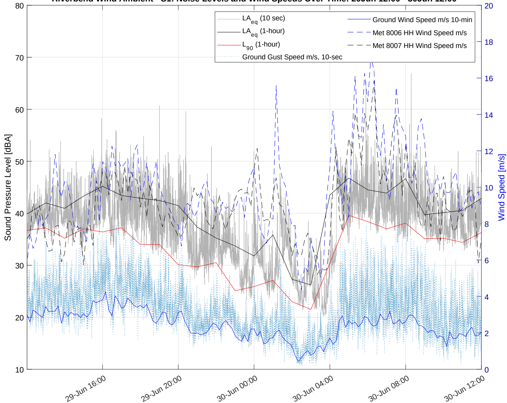
Riverbend Wind Ambient - S1: Noise Levels and Wind Speeds Over Time: 29Jun 12:00 - 30Jun 12:00
