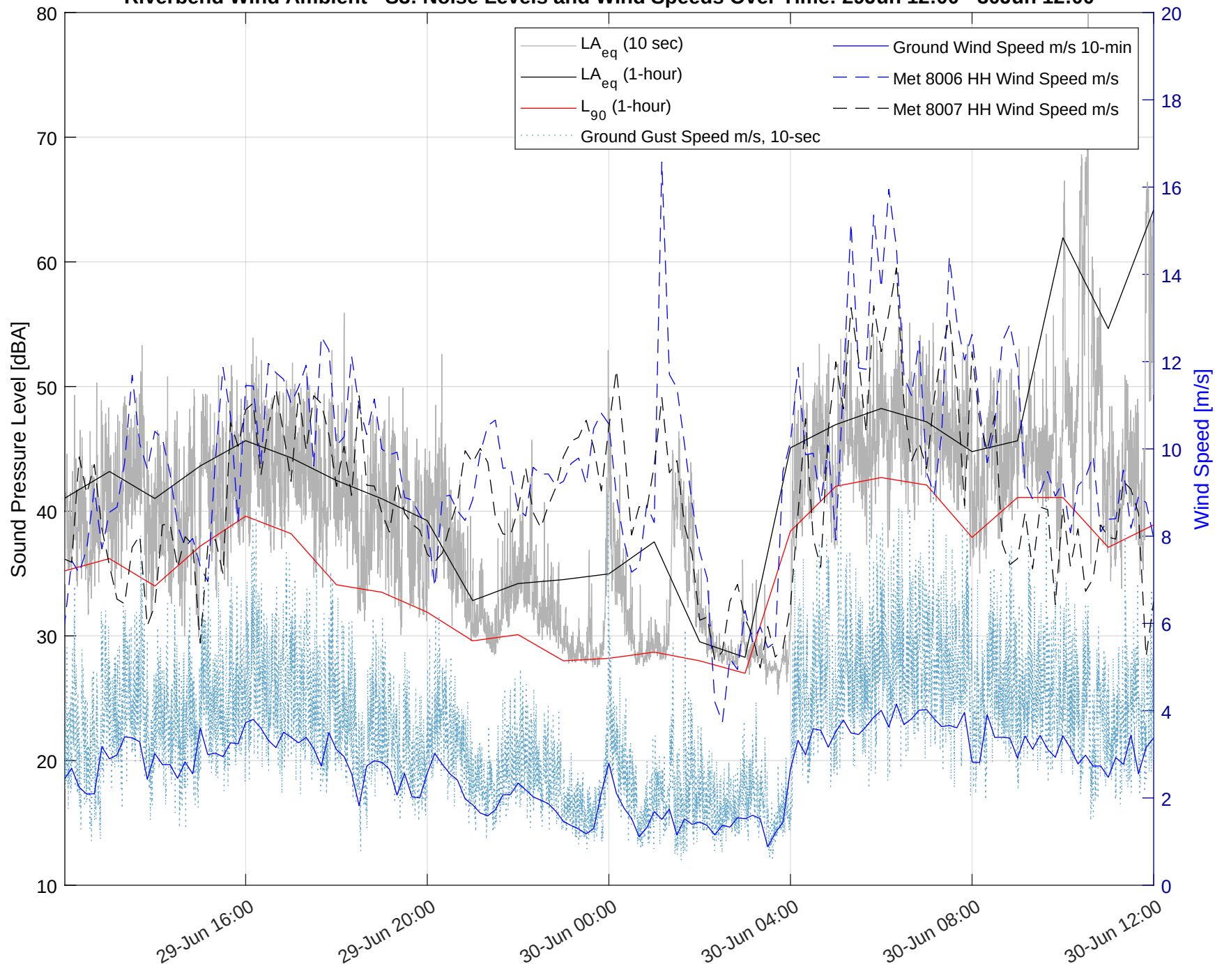
Riverbend Wind Ambient - S3: Noise Levels and Wind Speeds Over Time: 29Jun 12:00 - 30Jun 12:00
