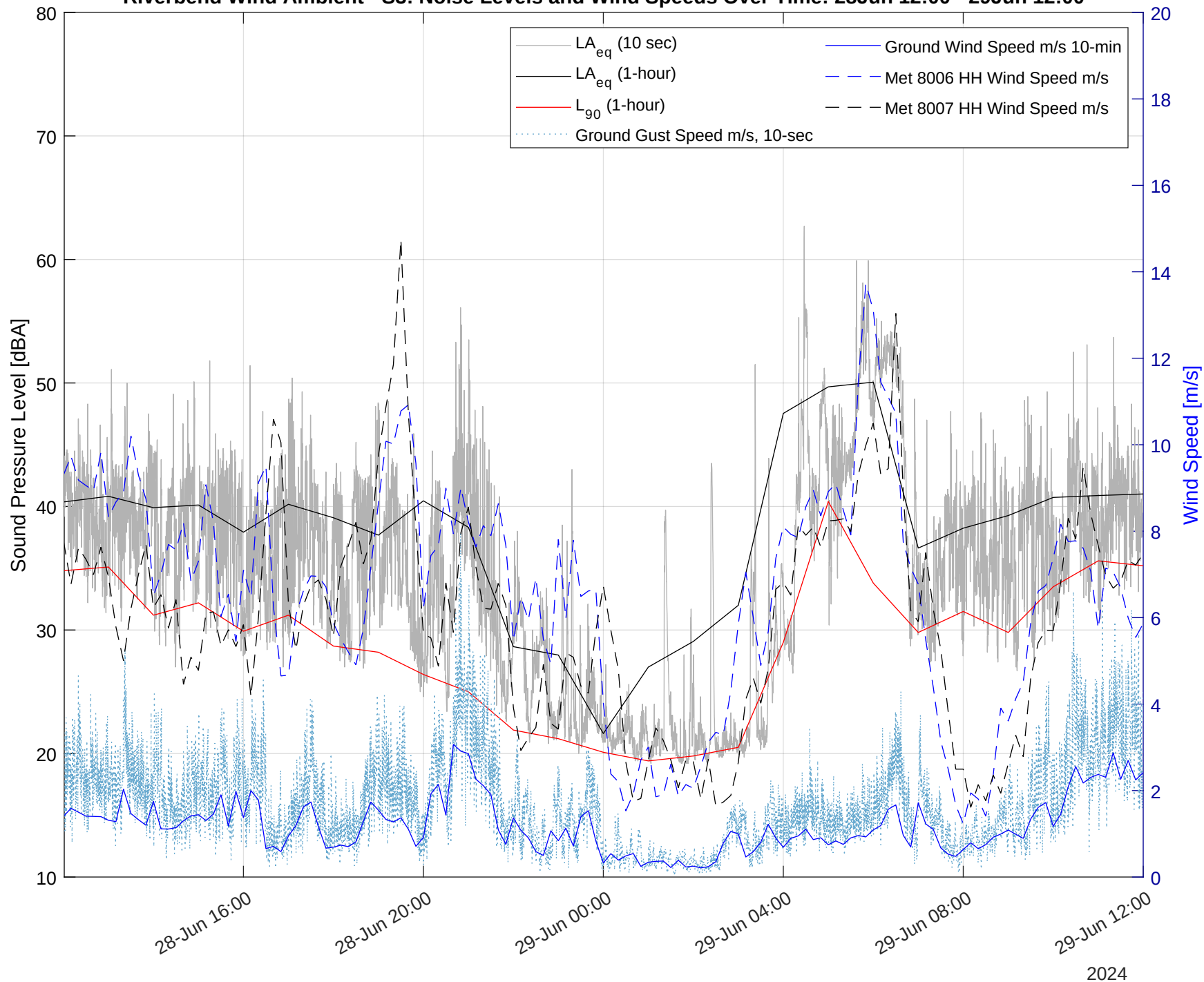
Riverbend Wind Ambient - S3: Noise Levels and Wind Speeds Over Time: 28Jun 12:00 - 29Jun 12:00
