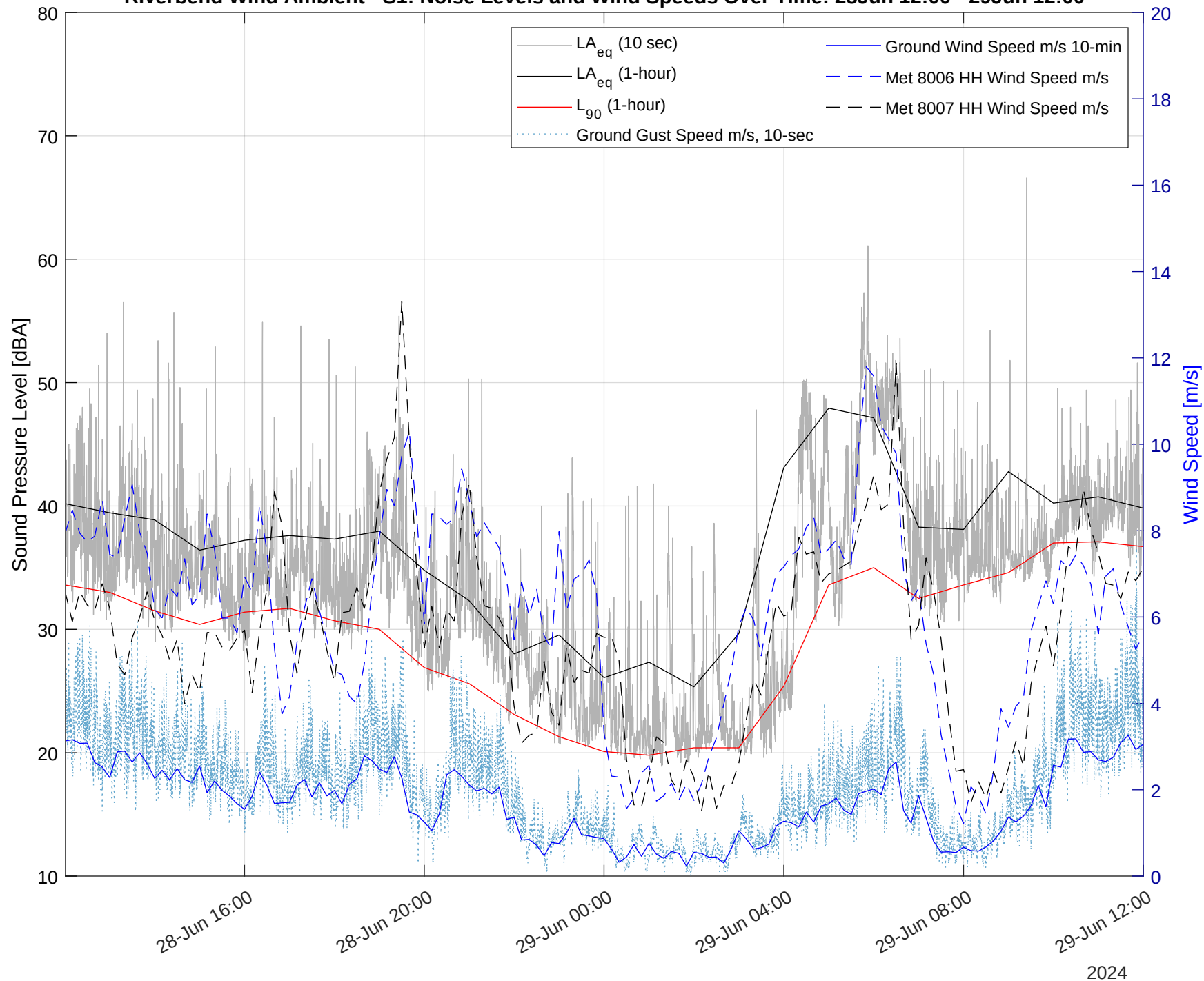
Riverbend Wind Ambient - S1: Noise Levels and Wind Speeds Over Time: 28Jun 12:00 - 29Jun 12:00
