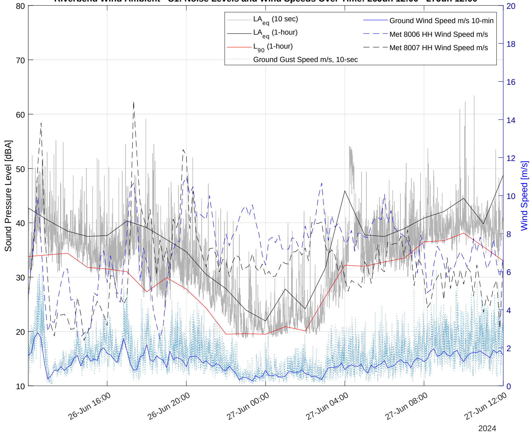
Riverbend Wind Ambient - S1: Noise Levels and Wind Speeds Over Time: 26Jun 12:00 - 27Jun 12:00
