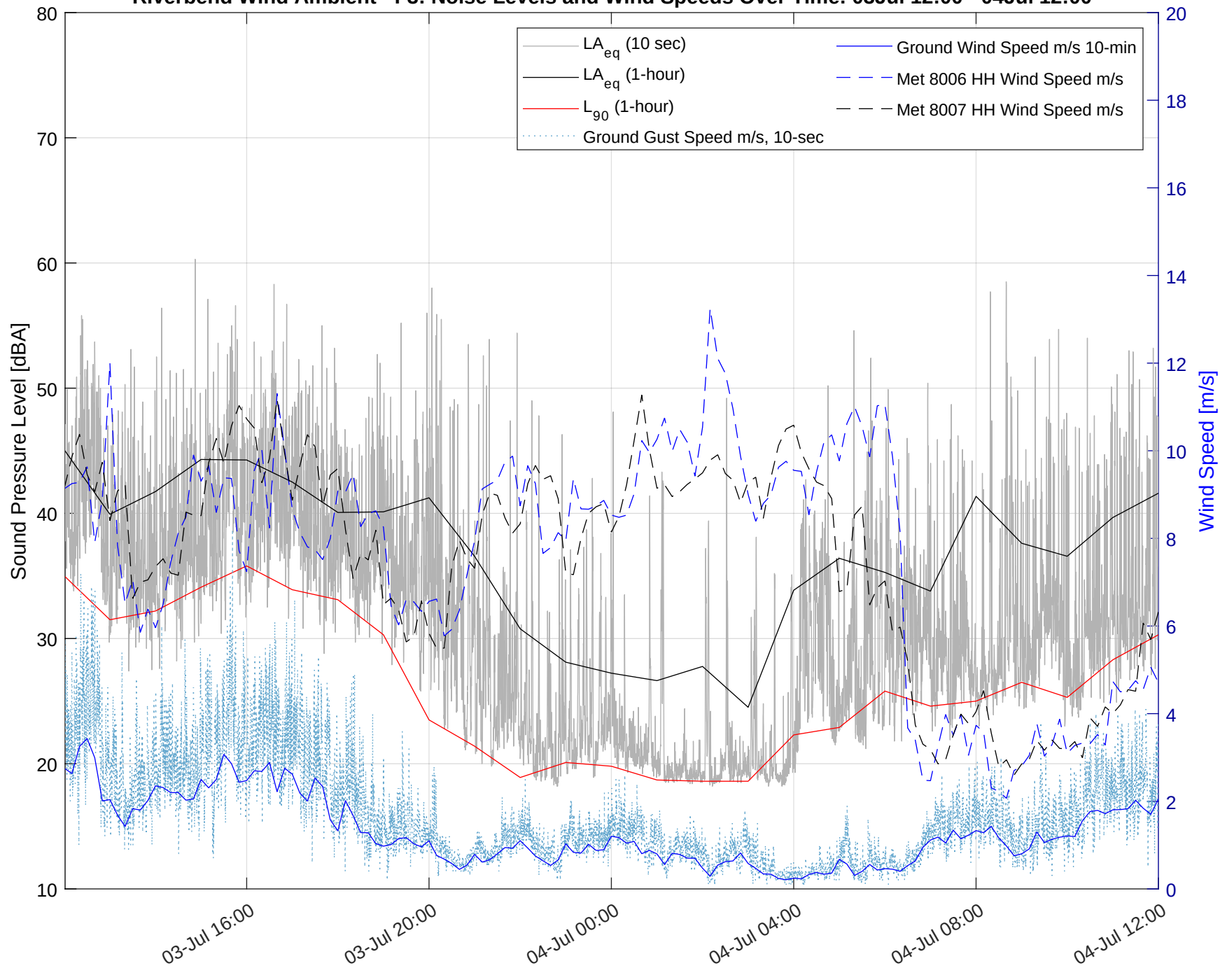
Riverbend Wind Ambient - F3: Noise Levels and Wind Speeds Over Time: 03Jul 12:00 - 04Jul 12:00
