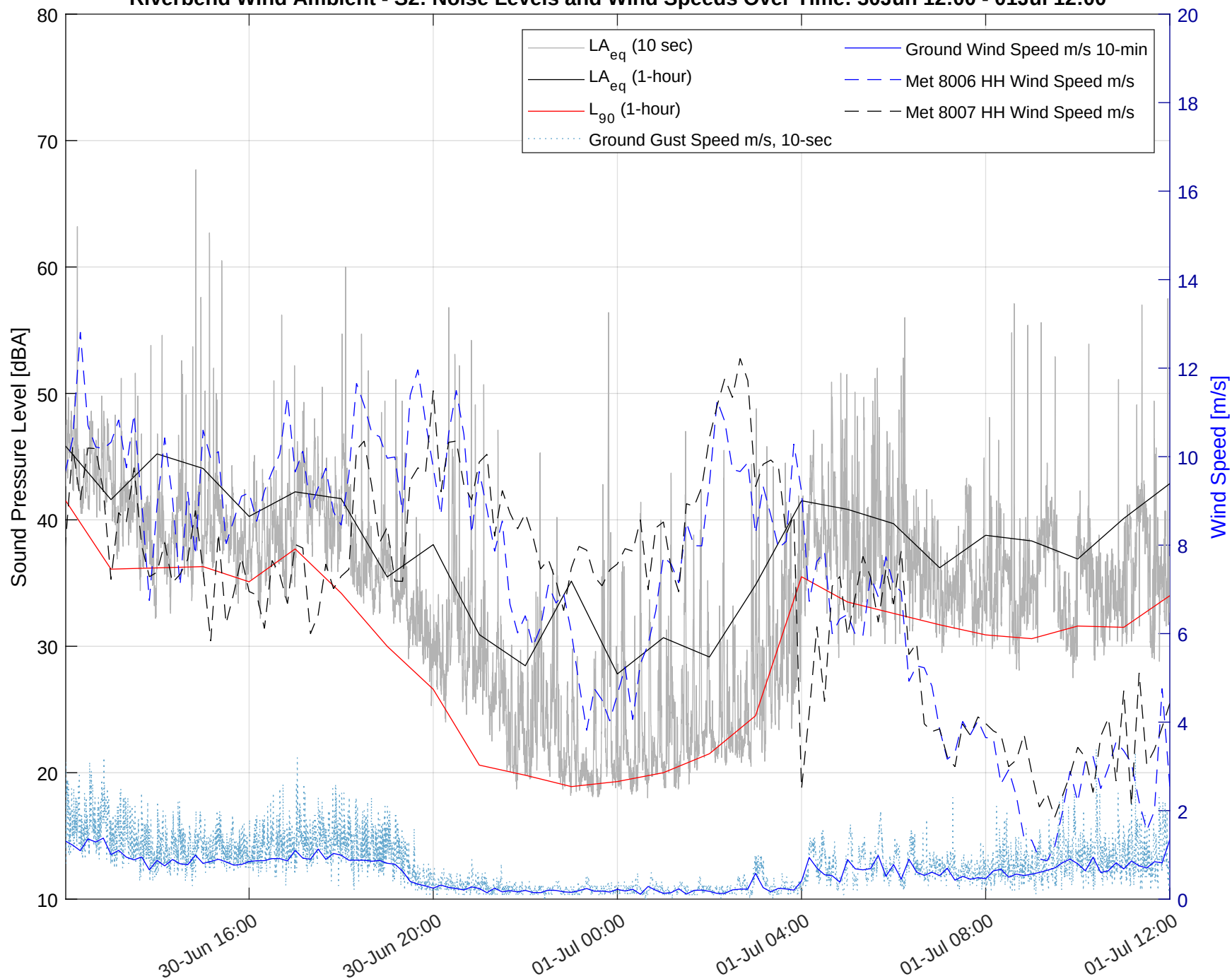
Riverbend Wind Ambient - S2: Noise Levels and Wind Speeds Over Time: 30Jun 12:00 - 01Jul 12:00
