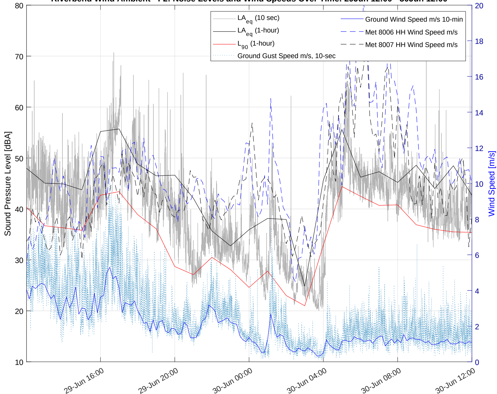
Riverbend Wind Ambient - F2: Noise Levels and Wind Speeds Over Time: 29Jun 12:00 - 30Jun 12:00
