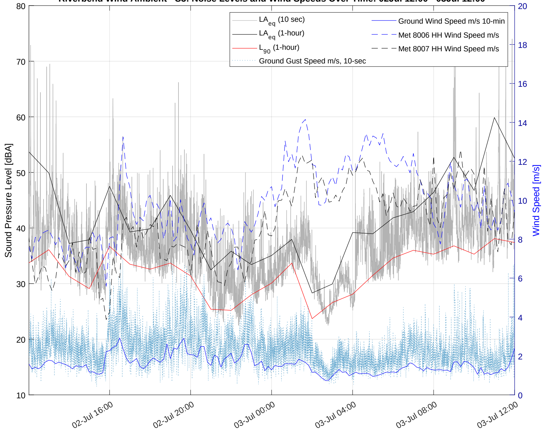
Riverbend Wind Ambient - S3: Noise Levels and Wind Speeds Over Time: 02Jul 12:00 - 03Jul 12:00
