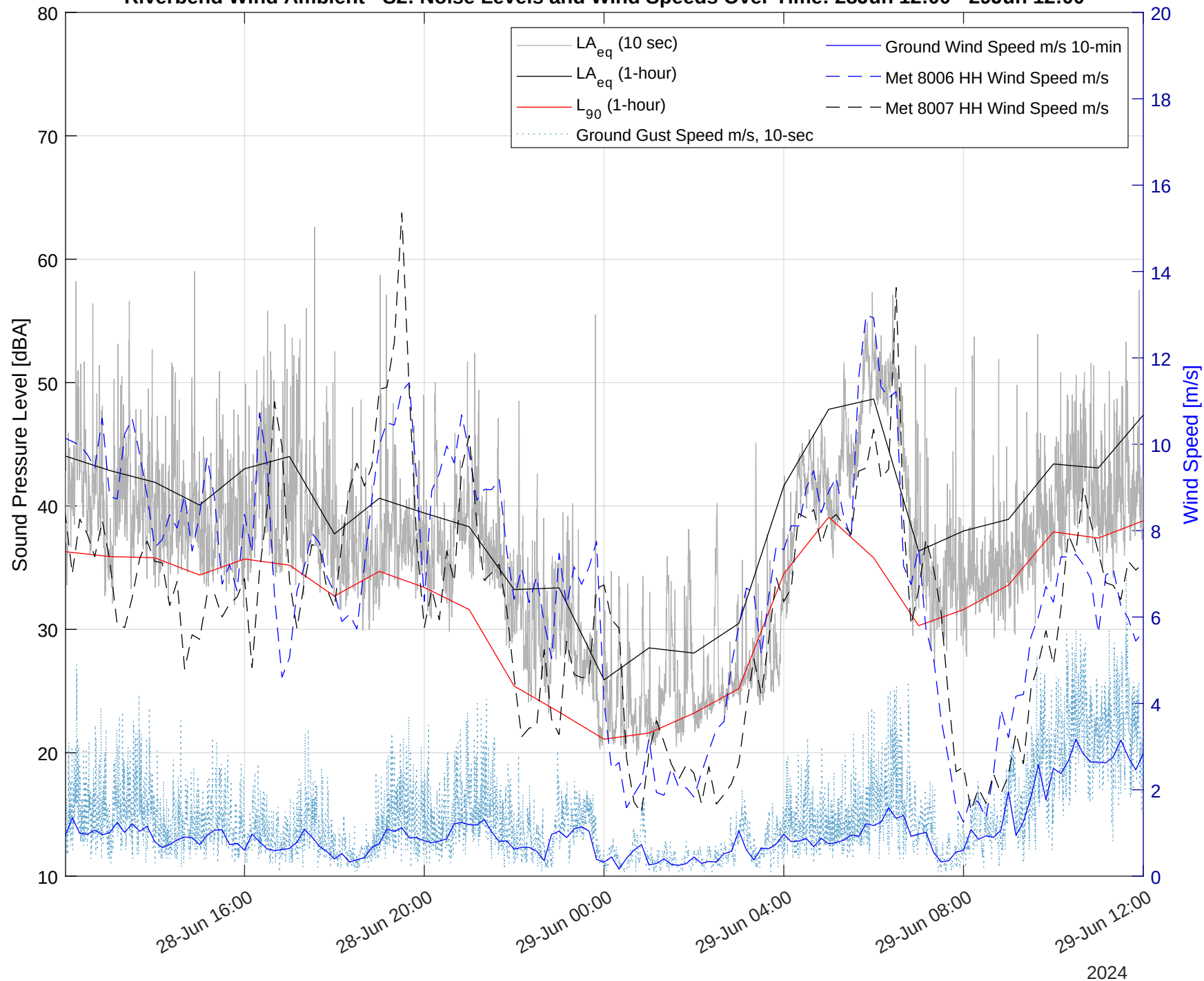
Riverbend Wind Ambient - S2: Noise Levels and Wind Speeds Over Time: 28Jun 12:00 - 29Jun 12:00
