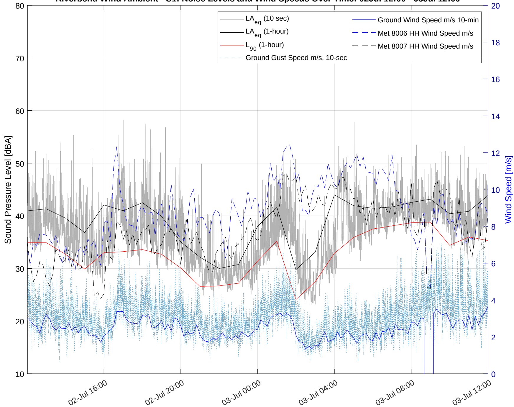
Riverbend Wind Ambient - S1: Noise Levels and Wind Speeds Over Time: 02Jul 12:00 - 03Jul 12:00
