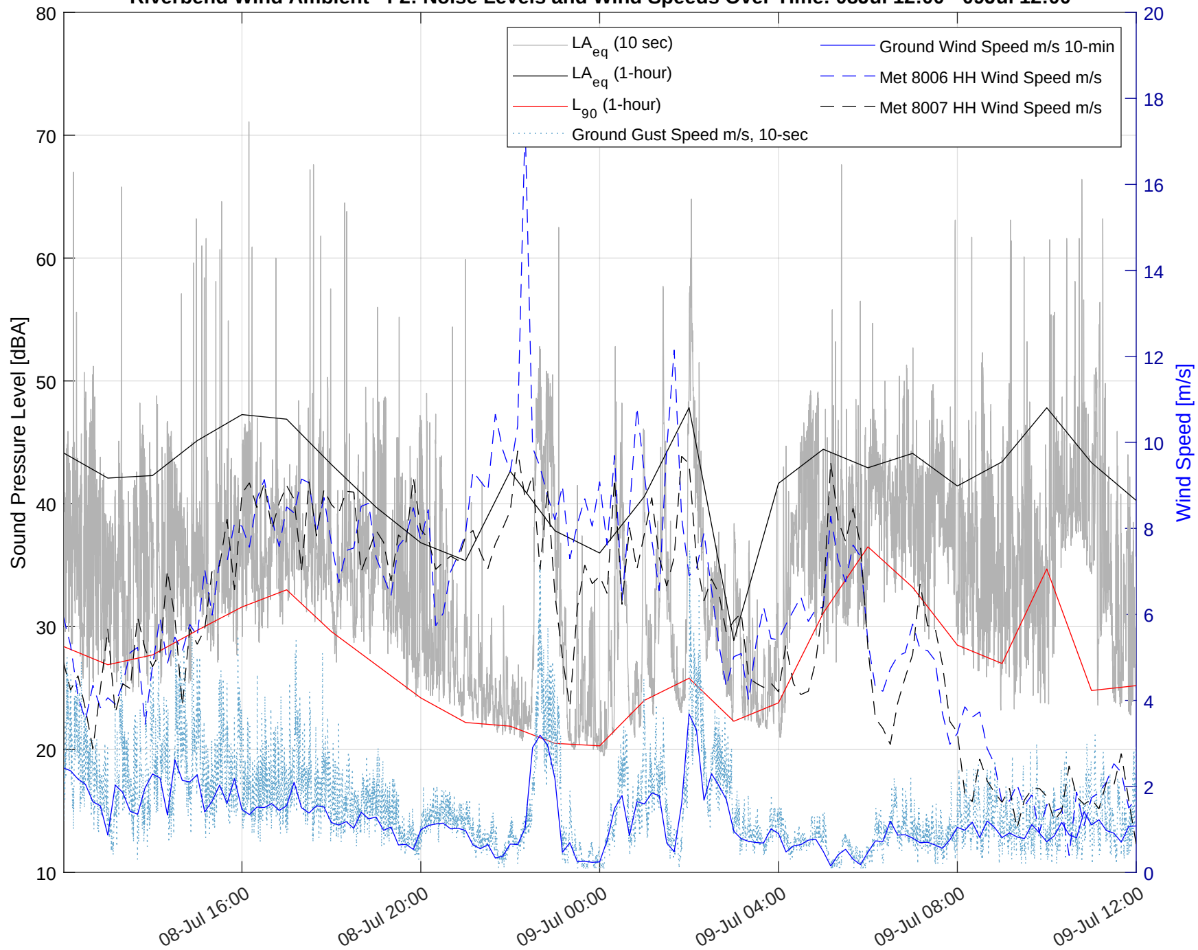
Riverbend Wind Ambient - F2: Noise Levels and Wind Speeds Over Time: 08Jul 12:00 - 09Jul 12:00
