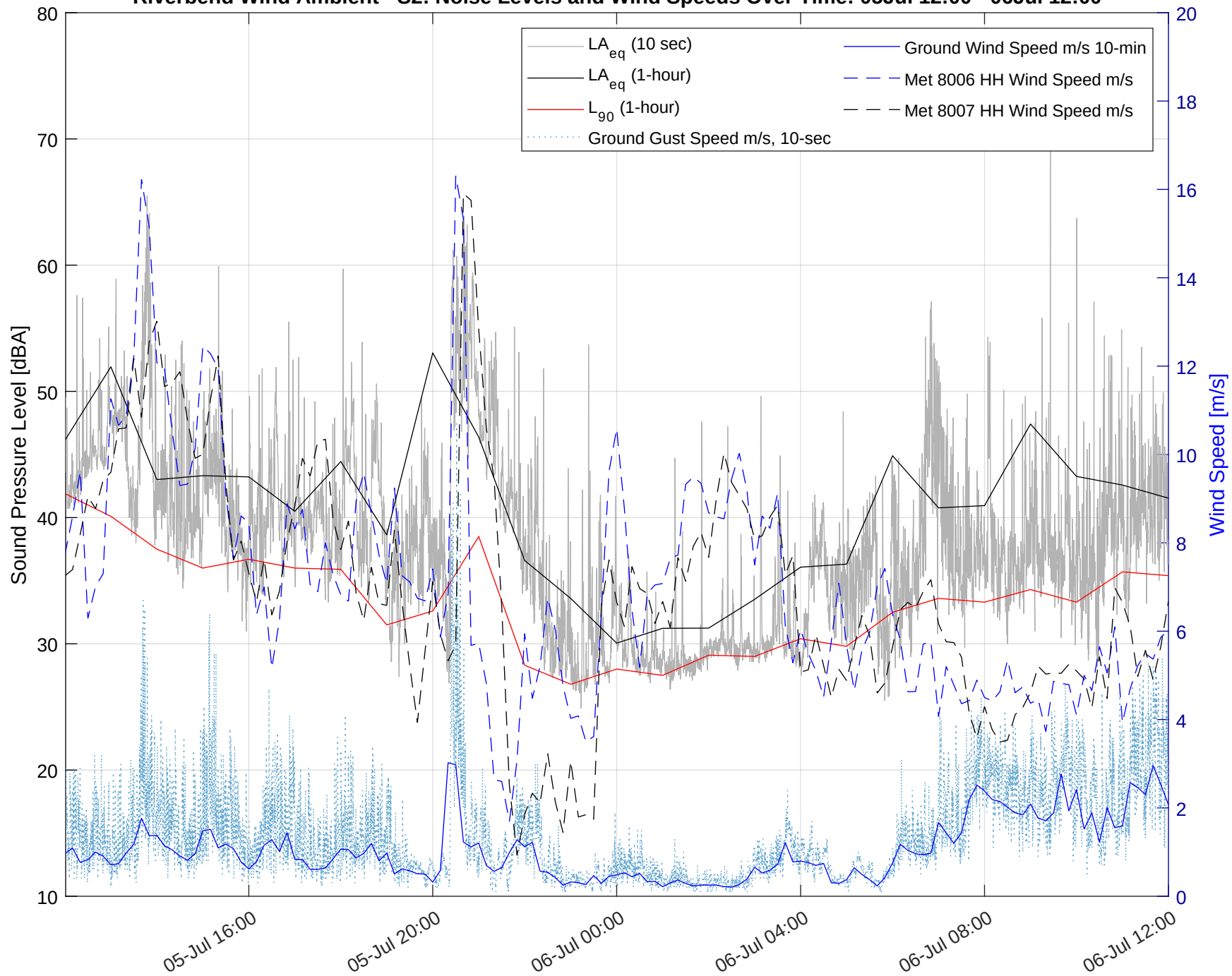
Riverbend Wind Ambient - S2: Noise Levels and Wind Speeds Over Time: 05Jul 12:00 - 06Jul 12:00
