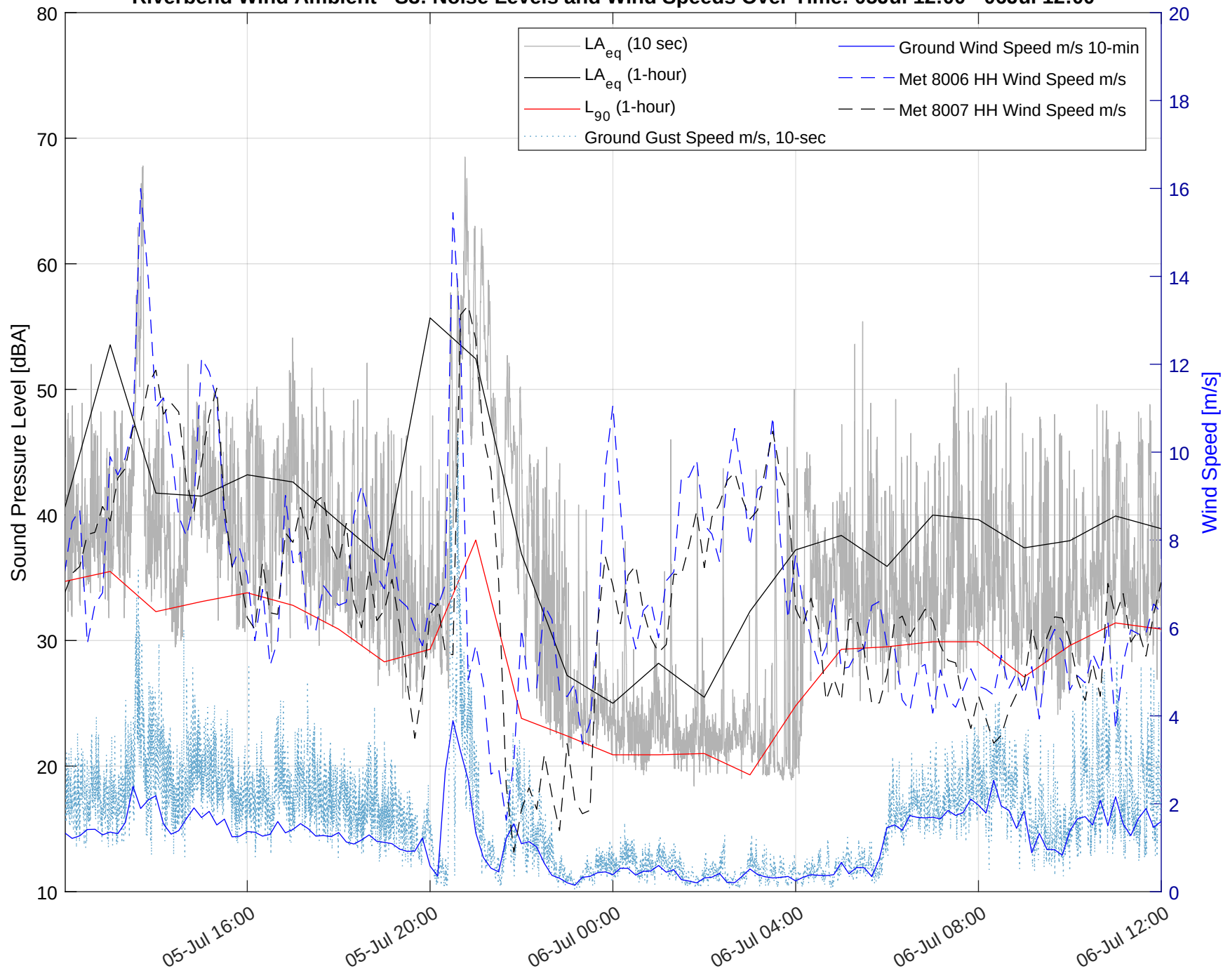
Riverbend Wind Ambient - S3: Noise Levels and Wind Speeds Over Time: 05Jul 12:00 - 06Jul 12:00
