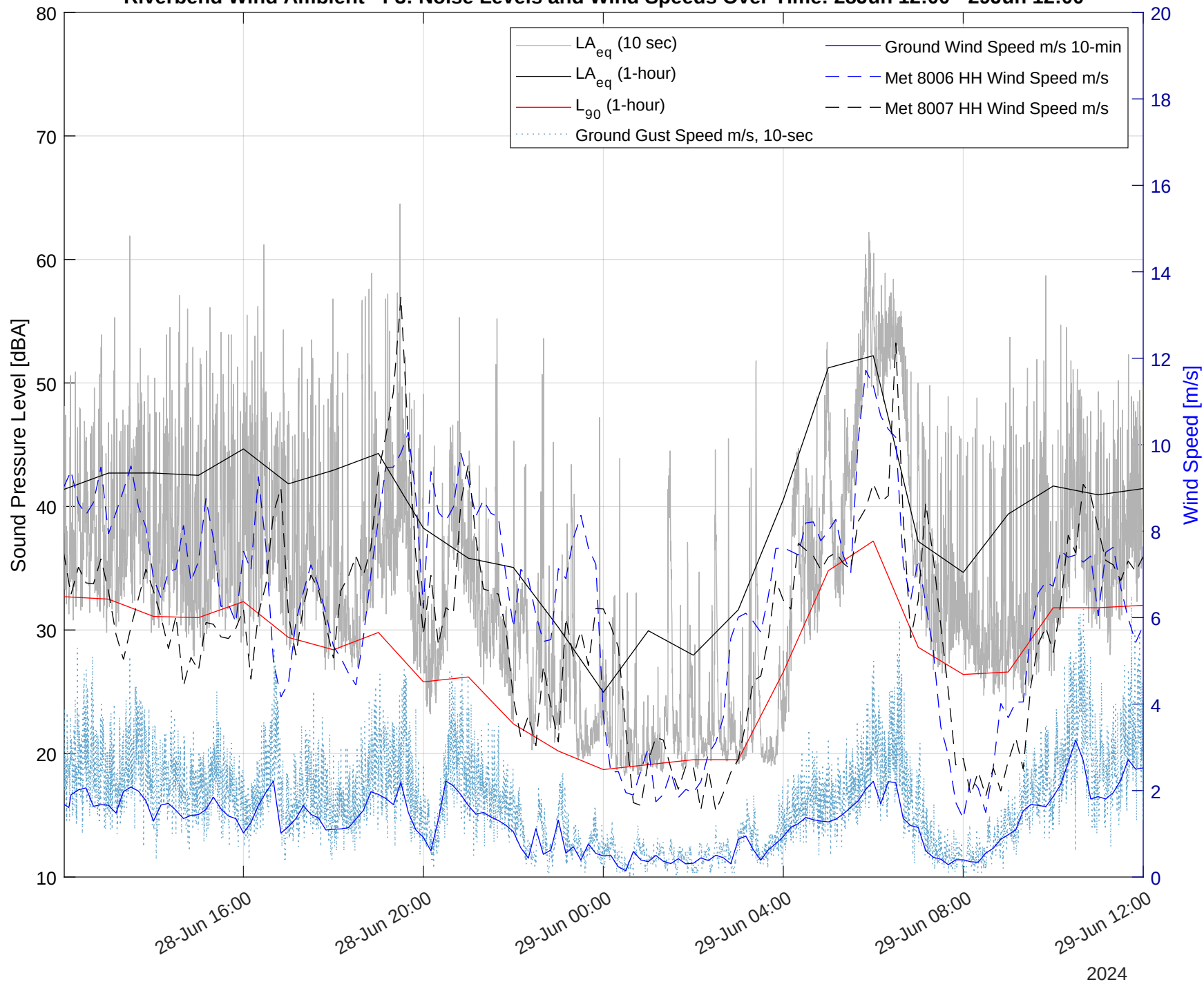
Riverbend Wind Ambient - F3: Noise Levels and Wind Speeds Over Time: 28Jun 12:00 - 29Jun 12:00
